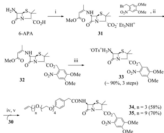
Scheme 5. Synthesis of Penicillin G photo-cleavable ester equipped with a side-chain for Si (Ge) surface-grafting.
