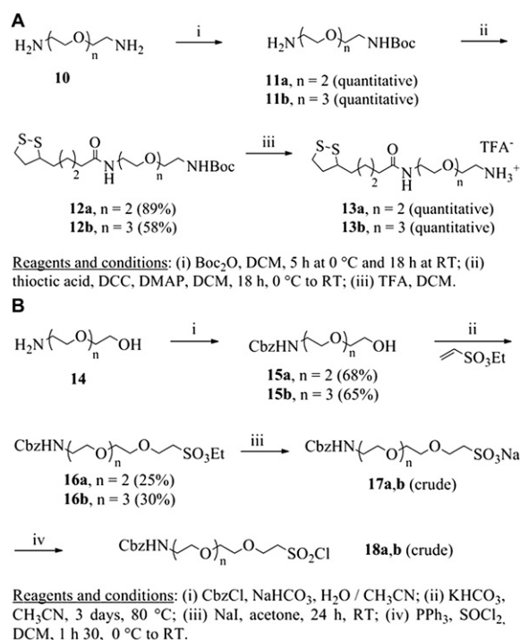
Scheme 2. Synthesis of spacer-arms (part I).
