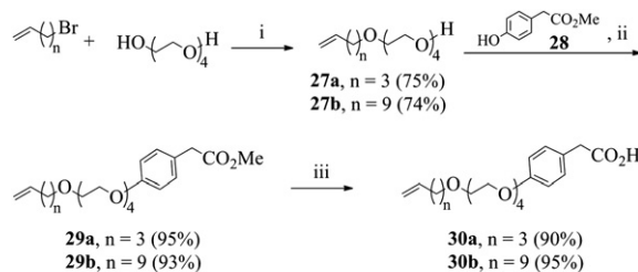
Scheme 4. Synthesis of spacer-arms (part II) coupled to the side-chain of Penicillin.
