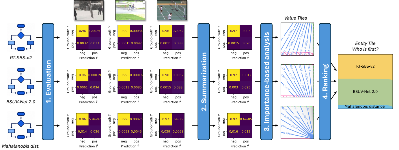
Fig. 6. Illustration of a complete pipeline for evaluating and comparing the performance of methods, applied to the task of background subtraction on CDnet. The pipeline consists of four steps: (1) evaluation : this step involves determining, for each method—as illustrated for the three methods RT-SBS-v2 [16], BSUV-Net 2.0 [17], and the Mahalanobis distance [18]—the confusion matrix for each video (see the first three columns); (2) summarization , which involves aggregating the confusion matrices into a mixture; (3) analysis of various scores based on application-related importances, represented graphically using Value Tiles; and (4) comparison of the methods using the Entity Tile. More information about Tiles can be found in Fig. 7.
