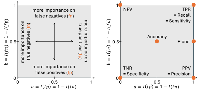
Fig. 7. Two interpretative readings of the Tile: a map of application-specific importances (left) and a map of scores to induce meaningful performance-based rankings (right) (taken from [40]).
