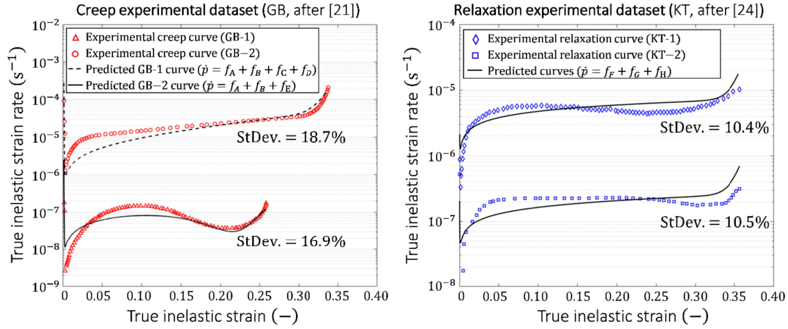
Fig. 6: Comparison of predicted and experimental \dot{p} - p curves of Incoloy 800H exhibiting non-classical creep and relaxation viscoplastic regimes.
