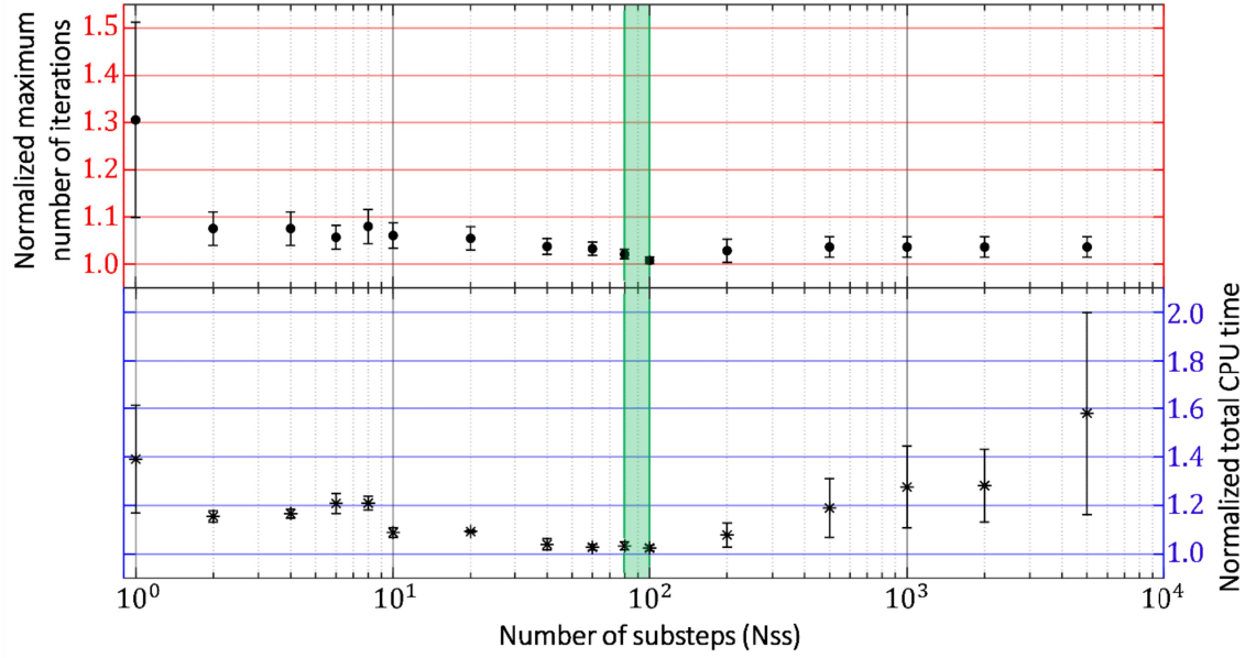
Fig. 7: Numerical and computational performance of the UVCN applied on non-classical viscous behavior of Incoloy 800H with a wide range of number of sub-steps (Nss). The green zone highlights the optimal Nss where the lowest number of iterations and lowest CPU time is achieved.
