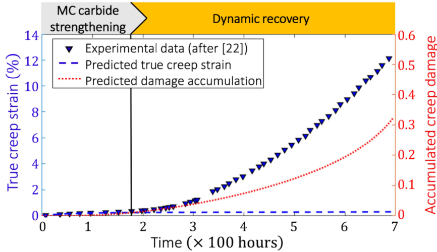
Fig. 2: True creep strain and damage accumulation predicted by a conventional Chaboche UVCN applied to non-classical creep behavior of 800H alloy.
