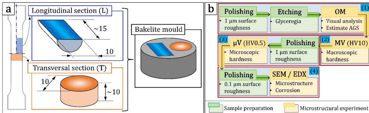
Figure 3 (a) Illustration of the cutting of 800H alloy specimens and mounting into bakelite moulds. (b) Flowchart describing the microstructural characterization campaign conducted per each in-bakelite specimen.
