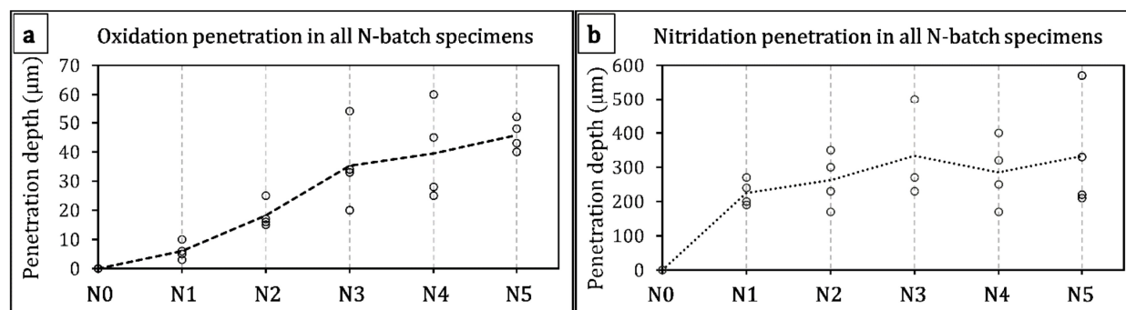
Figure 10 Measured oxidation (a) and nitridation (b) penetration depth into the material based on microstructural observations of the deepest found corrosion-related precipitate. The hollow circular points indicate the maximum depth measured at each edge zone of interest (zones E1 to E4, see Figure 7a).
