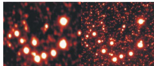
20" region (Left) with ISAAC. (Right) with MAD-GLAO.
