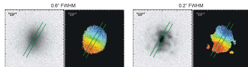
Simulation of a galaxy, slit of 0.25". ARGOS PDR
