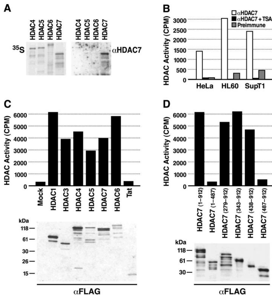
FIG. 3. Mapping human HDAC7-associated HDAC activity to a carboxyl-terminal domain. A, characterization of a polyclonal anti-HDAC7 antiserum. cDNAs for HDAC4, 5, 6, and 7 were translated in vitro using [ ^{35}\text{S} ]methionine. The corresponding recombinant proteins were separated by SDS-PAGE and transferred to a nitrocellulose membrane. The left panel shows the equal loading of all class II HDACs on the membrane by autoradiography ( ^{35}\text{S} ). The right panel shows Western blot analysis of the same membrane with our polyclonal anti-HDAC7 antiserum ( \alpha\text{HDAC7} ) or the corresponding preimmune serum. The HDAC activity of immunoprecipitates was measured with a radiolabeled histone H4 peptide in the absence or presence of 400 nM TSA. The enzymatic activity represents the average of three independent experiments. C, vectors encoding HDAC1, 3, 4, 5, 6, and 7 and the HIV Tat protein (all proteins tagged with the FLAG epitope) or the empty vector as control were transiently transfected into 293 cells. Fusion proteins were immunoprecipitated with anti-FLAG antiserum and tested for HDAC activity. The activity is presented as the average of three independent experiments. To control for the expression level and the efficiency of the immunoprecipitation, the immunoprecipitated material was analyzed by Western blotting with specific antisera against the FLAG epitope ( \alpha\text{FLAG} ). D, the indicated FLAG-tagged constructs corresponding to full-length HDAC7 or to amino- or carboxyl-terminal deletions of HDAC7 were transiently transfected into 293 cells. Material immunoprecipitated with the anti-FLAG antiserum was tested for HDAC activity. Western blotting of the immunoprecipitated material with a specific anti-FLAG antiserum was performed to control for the expression level of the transfected constructs ( \alpha\text{FLAG} ).
