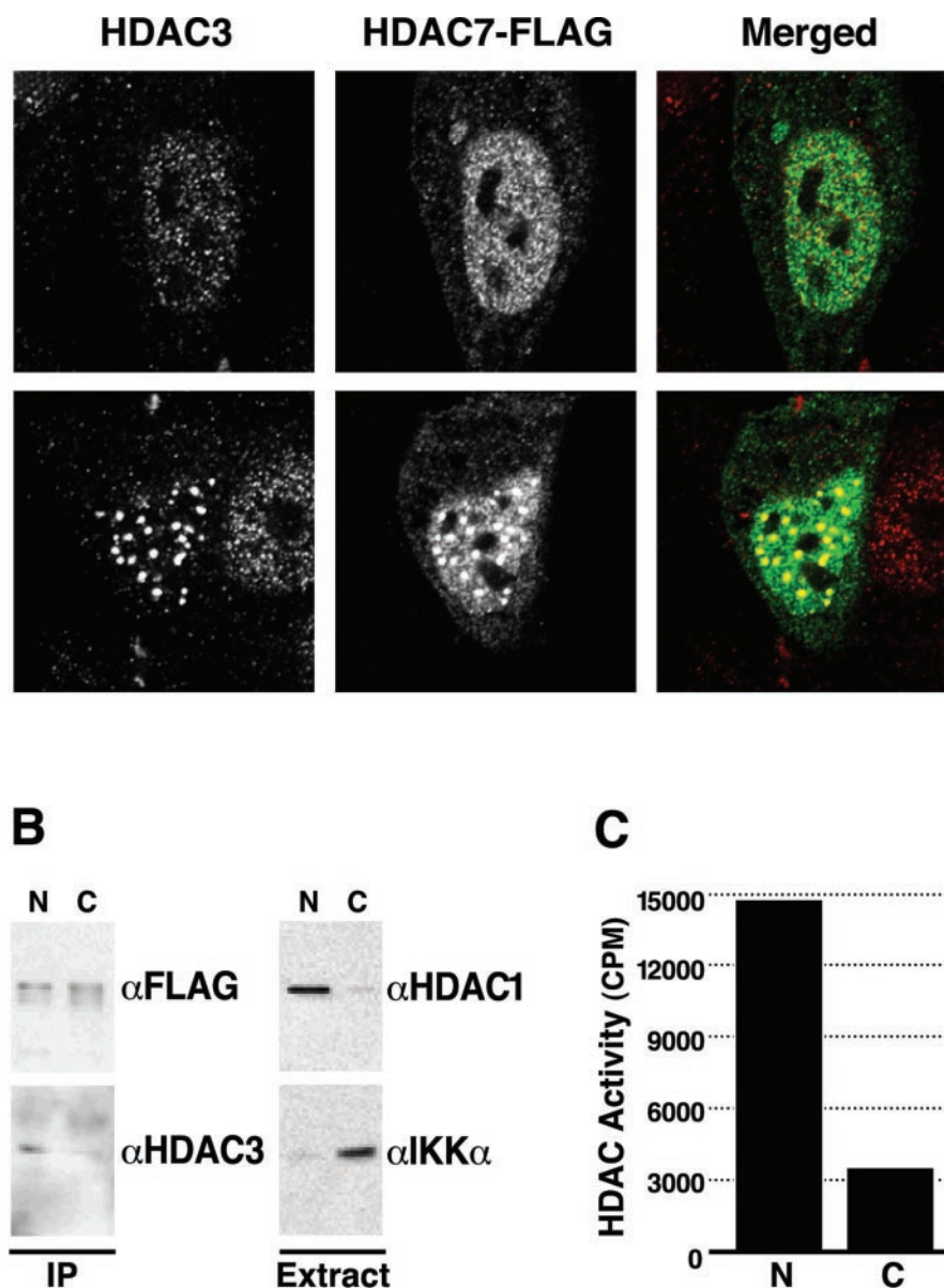
FIG. 5. Nuclear HDAC7 bound to HDAC3 is associated with enzymatic activity, whereas free cytoplasmic HDAC7 is inactive. A, HeLa cells were transiently transfected with an expression vector encoding HDAC7-FLAG. Endogenous HDAC3 was detected with affinity-purified anti-HDAC3 antibodies combined with a Cy3-labeled secondary antibody (red). FLAG-tagged HDAC7 was visualized with the M2 antibody in combination with an Alexa 488-tagged secondary antibody (green). For better visualization of the expression intensities of the individual HDACs, black and white images are shown. The yellow dots in the merged image indicate colocalization of both factors. Two different cells representing different expression levels and nuclear distribution profiles are shown. B, nuclear (lanes N) and cytoplasmic (lanes C) extracts were prepared from 293 cells transiently transfected with HDAC7-FLAG. Both extracts were immunoprecipitated (IP) with anti-FLAG antiserum, and bound material was analyzed by Western blotting with antisera against the FLAG epitope ( \alpha FLAG) and HDAC3 ( \alpha HDAC3). Extracts were also directly analyzed using Western blotting with antisera against the cytoplasmic protein IKK \alpha ( \alpha IKK \alpha ) and the nuclear protein HDAC1 ( \alpha HDAC1). C, activity associated with HDAC7 from nuclear extracts (N) and cytoplasmic extracts (C) after immunoprecipitation of HDAC7-FLAG.
