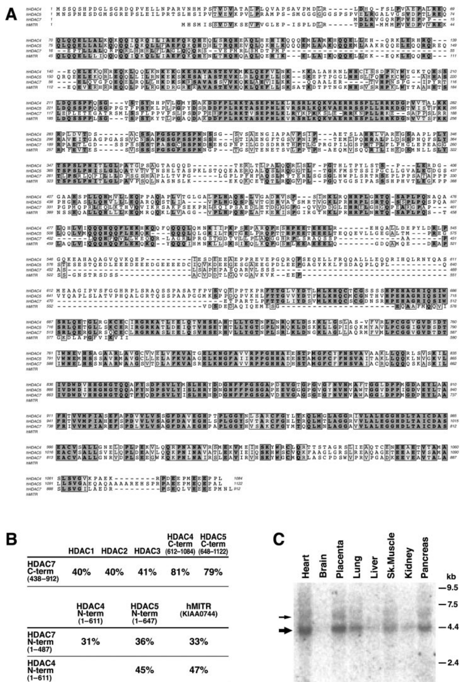
FIG. 1. hHDAC7 is a human class II HDAC. A, an alignment of the predicted amino acid sequences of human HDAC4, HDAC5, HDAC7, and MITR was created with the ClustalW routine of the MacVector program. Identical amino acids are shaded; related amino acids are boxed. B, degree of similarity between different HDACs. The percentages refer to the homology of amino acid sequences in the amino-terminal domains (N-term) or the carboxyl-terminal HDA1-like regions (C-term) and were calculated based on the alignment shown in A. C, expression profile of human HDAC7 mRNA. A multiple human tissue Northern blot was probed with the HDAC7 cDNA. The arrows indicate the major mRNA species of ~4.4 kb and a putative alternatively spliced species of ~6.0 kb. Molecular size markers are indicated on the right.
