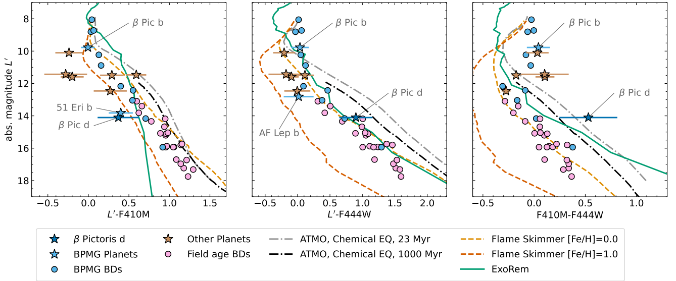
Figure 5. CMDs of \beta Pic d, shown alongside photometry for directly imaged planets in BPMG (blue stars) and around other stars (brown stars), as well as free-floating brown dwarfs in BPMG (blue circles) and the field (pink circles). While young (BPMG) and field-age brown dwarfs have similar colors as a function of magnitude, the planets are markedly fainter at F410M than brown dwarfs with comparable magnitude. We show evolutionary models from ATMO (M. W. Phillips et al. 2020) and atmosphere models from Sonora Flame Skimmer (J. Mang et al. 2026 in preparation) and ExoRem (J.-L. Baudino et al. 2015; B. Charnay et al. 2018). For the atmosphere models, we assume \log g = 4.0 dex and R = 1.3 R_{\text{Jup}} . Sonora Flame Skimmer models adopt solar C/O, K_{zz} = 4 , and two metallicities ( [\text{Fe}/\text{H}] = 0.0 and 1.0 ), while the ExoRem model has [\text{Fe}/\text{H}] = 0.5 , \text{C}/\text{O} = 0.65 , and is chosen based on the best-fit model of 51 Eri b in W. O. Balmer et al. (2025b); this model also provides the closest match to \beta Pic d of all models shown.
