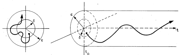
Figure 2. Illustration of the definition of stability [57].
