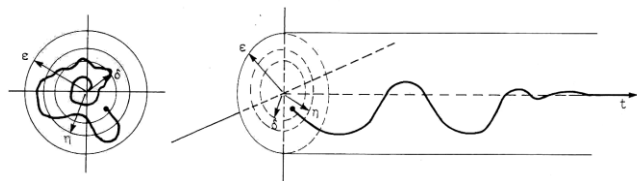
Figure 3. Illustration of the definition of asymptotic stability [57].
