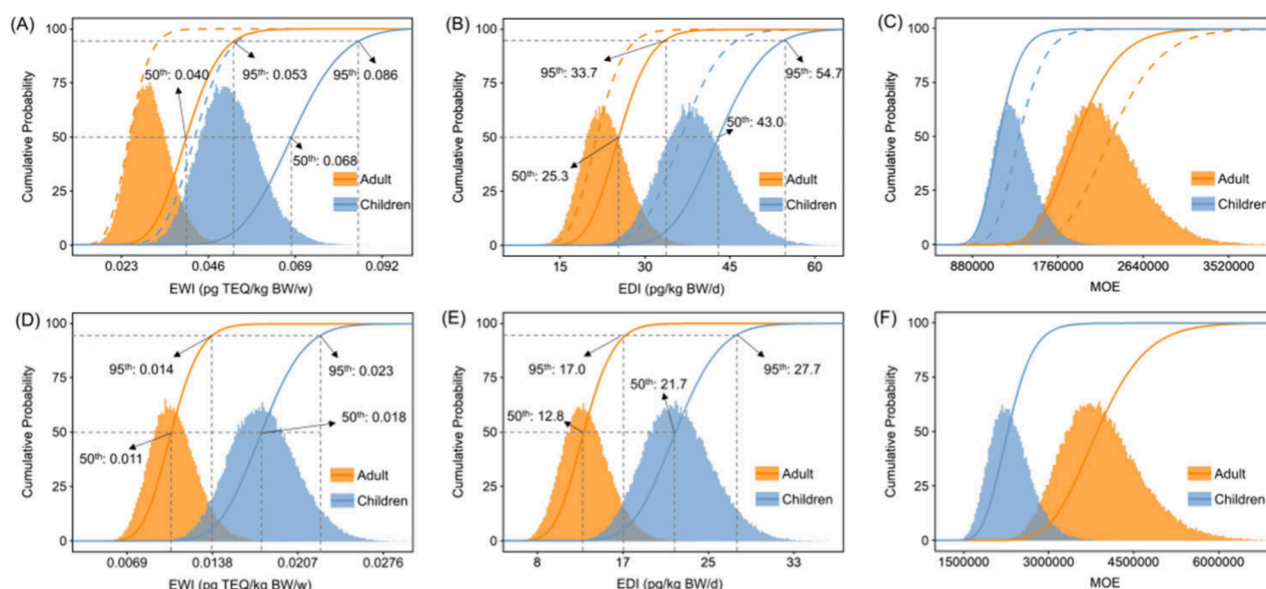
Figure 5. Risk assessment of resident's exposure to PCNs through poultry egg consumption. Probability density distributions of estimated weekly intake (EWI) of PCN TEQs for adults and children in (A) Hunan Province and (D) Guangxi Province (solid line curve for waterfowl eggs; dashed line for chicken eggs). Probability density distributions of estimated daily intake (EDI) of PCNs for adults and children in (B) Hunan Province and (E) Guangxi Province. Probability density distributions of margin of exposure (MOE) of PCNs for adults and children in (C) Hunan Province and (F) Guangxi Province.
