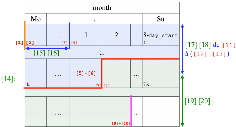
Figure 25. The fill-in-the-blank GLI for solving the second problem (Display a calendar).
