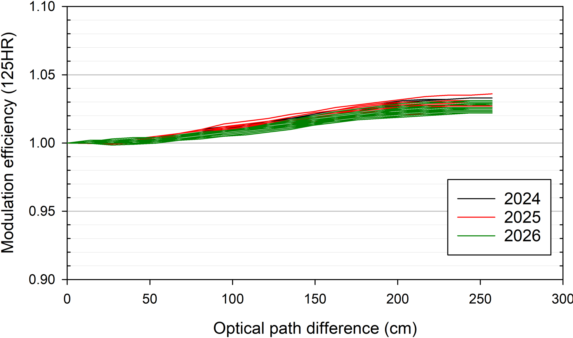
Figure 3. Modulation efficiency derived with Linefit v14.5 from the fit of 14 HBr lines. Laboratory spectra have been recorded regularly since instrument deployment in September 2024 with the HBr cell #7. Supplemental spectra have been recorded with HBr cells #54 and #55 as well as with the \text{N}_2\text{O} cell #117; they are currently being analyzed.
