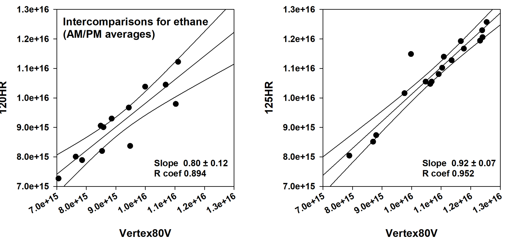
Figure 5. Scatter plots showing the 120HR vs Vertex and 125HR vs Vertex intercomparisons for ethane (upper panels), and carbon monoxide (bottom panels), considering AM/PM averages.
