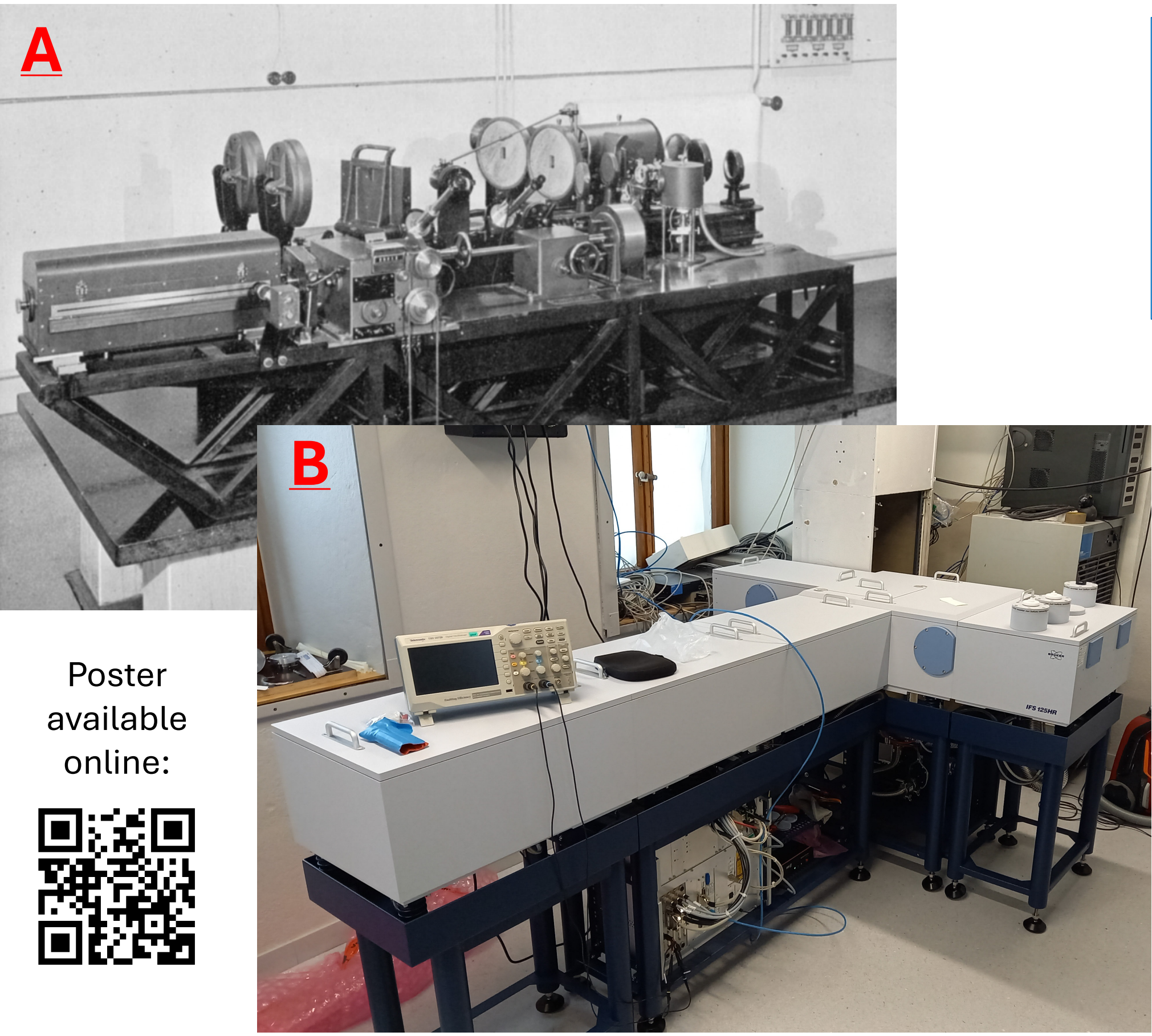
Figure 1. Panel A: The grating instrument developed and used at Jungfraujoch by Pr Marcel Migeotte in the early 1950s. Panel B: the new 125HR instrument soon after its installation in the FTIR laboratory (September 2024).
