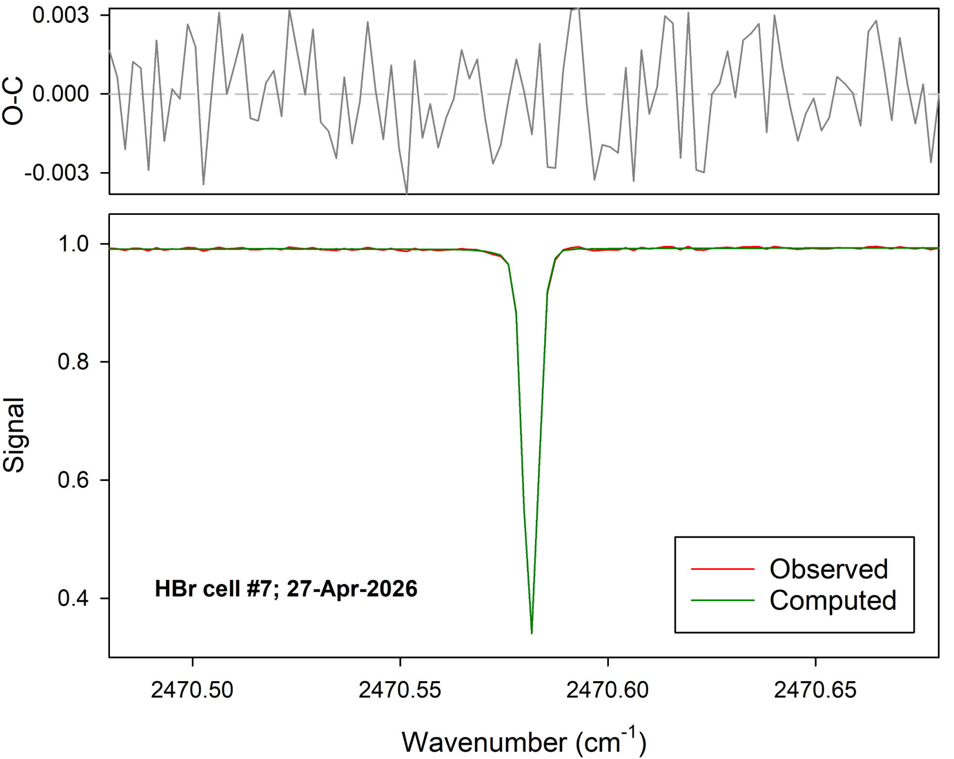
Figure 4. Fit to the HBr line at 2470.58 \text{cm}^{-1} for a laboratory spectrum recorded on April 27, 2026, with the 125HR spectrometer.
