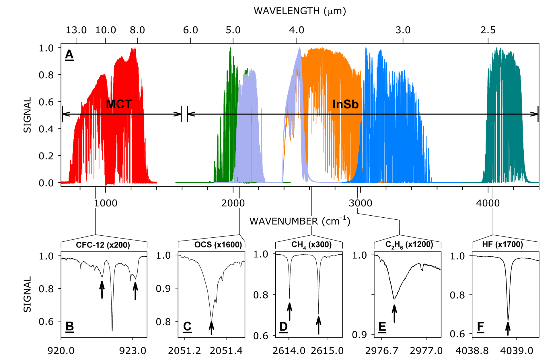
Figure 2. Panel A: the spectral ranges covered by the 125HR instrumental setup, involving two cooled detectors. The six optical filter band-paths are color-coded. Panels B-F show, after scaling the horizontal axis by 200 to 1700, a selection of spectral micro-windows that include absorption bands of several target molecules. Mind the different vertical scales.
