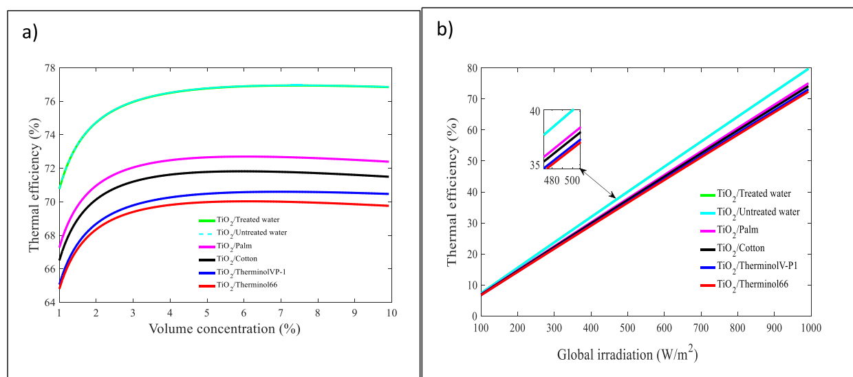
Fig. 12. Variation of thermal efficiency as a function of volume concentration (a) and solar irradiation (b).
