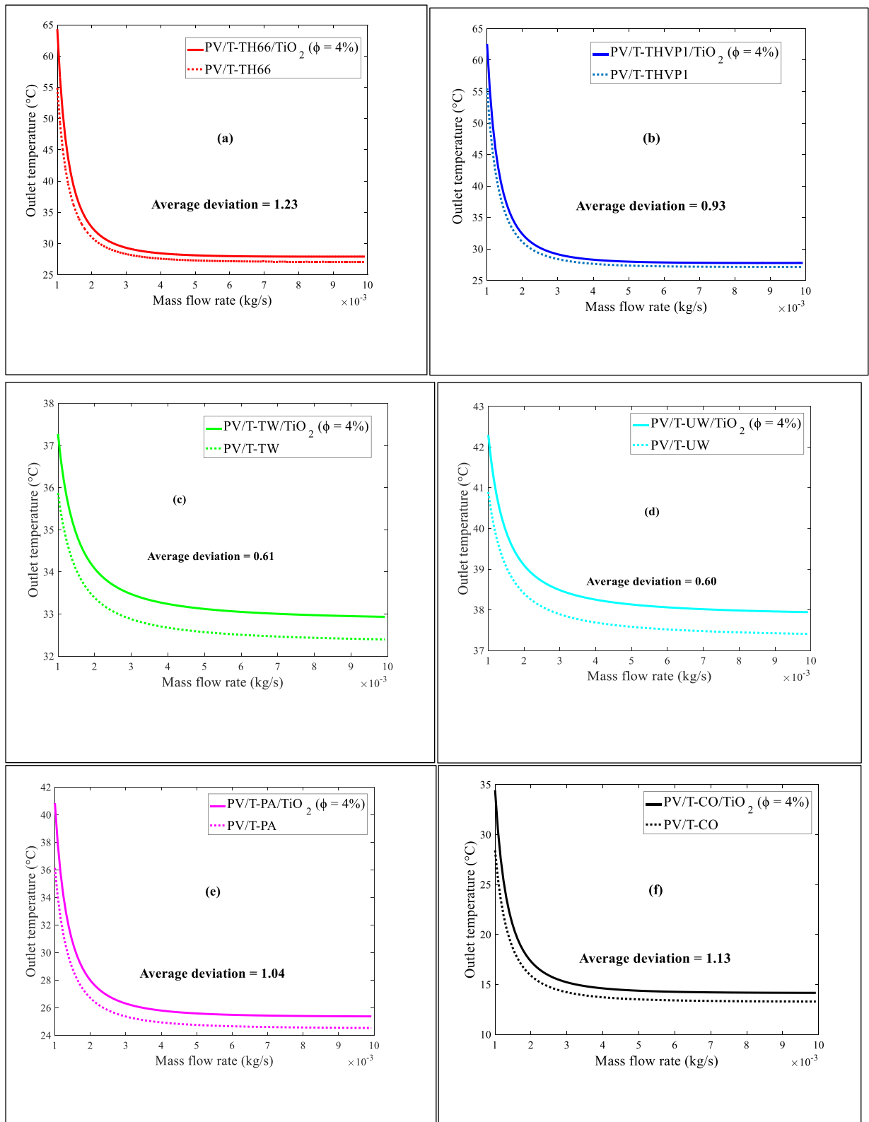
Fig. 10. Variation of fluid outlet temperature for PV/T configurations of TH66 (a), THVP1 (b), TW (c), UW (d), PA (e) and CO (f) with and without TiO 2 as a function of mass flow.
