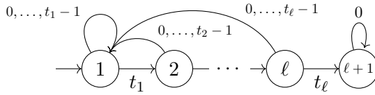
Figure 1.6: Automaton accepting all factors of words in the noncanonical \beta -shift S'_\beta when \beta is a simple Parry number, with d_\beta(1) = t_1 t_2 \cdots t_l 0^\omega
