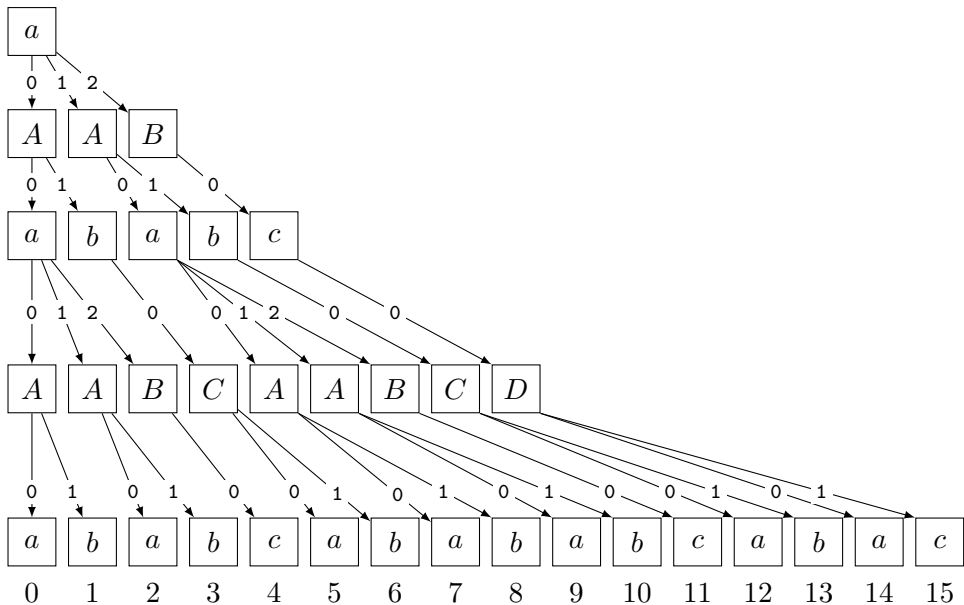
Figure 2.4: First levels of the tree \mathcal{T}_{\mu,a} .
