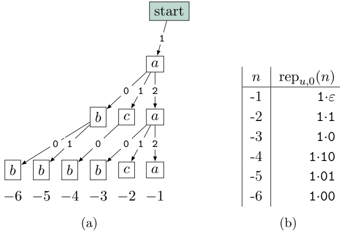
Figure 7.5: The tree \mathcal{T}_{\mu,a|} and the first few representations of negative integers in the numeration system associated with the substitution \mu: a \mapsto bca, b \mapsto bb, c \mapsto b , the left-infinite periodic point \mathbf{u} = \cdots bbca and residue r = 0 .
