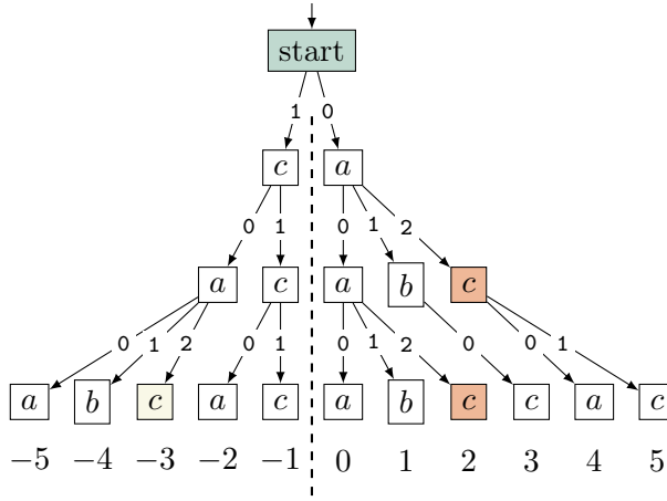
Figure 7.1: The tree \mathcal{T}_{\mu, c|a} associated with the two-sided periodic point \mathbf{u} of the substitution \mu: a \mapsto abc, b \mapsto c, c \mapsto ac with growing seed c|a .
