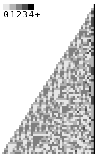
(a) Suffixes \omega(\text{rep}_U(U_n - 1)) in item 9.1b in Figure 9.1.
