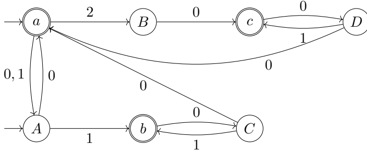
Figure 2.3: Automaton \mathcal{A} built from the words \lim_{n \rightarrow \infty} \text{rep}_U(U_{2n} - 1) and \lim_{n \rightarrow \infty} \text{rep}_U(U_{2n+1} - 1) .
