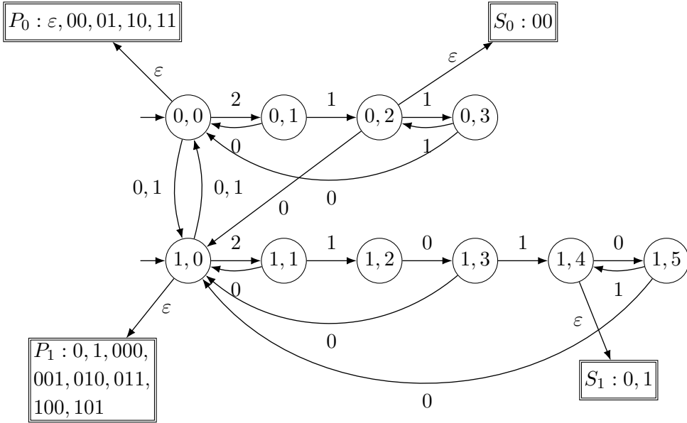
Figure 6.2: The nondeterministic automaton \mathcal{A} built from the set of maximal words M = 21(11)^*00 \cup 2101(01)^*1 \cup \{\varepsilon, 1, 11, 101\} .
