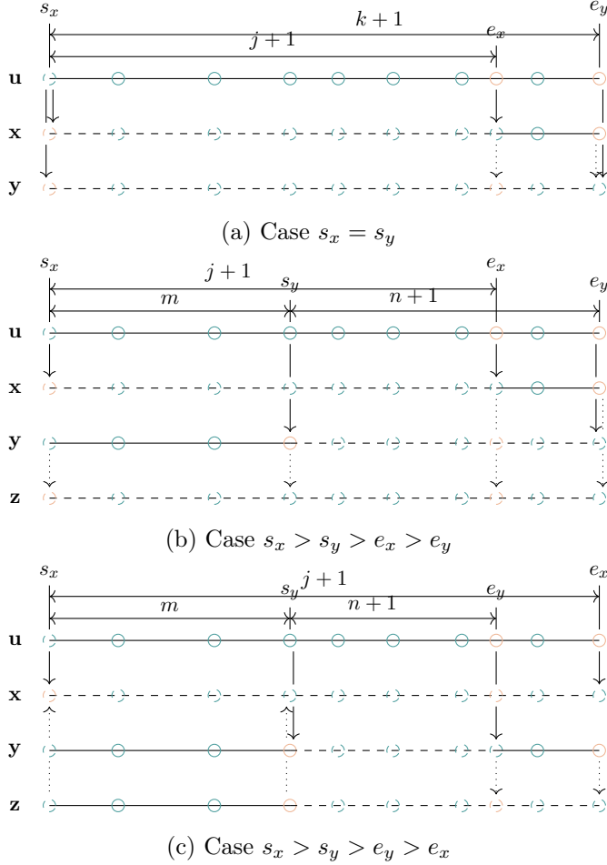
Figure 5.2: Visual representation for the proof of Lemma 5.36. Segments represent a "block" of the form d'_i or d_i . Continuous segments and nodes represent "big" digits, of the form d_{\cdot,\cdot} or t_{\cdot,\cdot} . Dashed segments and nodes represent "small" digits, being 0 or 1. Teal nodes correspond to the smaller of two possibilities, red nodes to the bigger of the two. Arrows indicate a rewriting, with \mathbf{u} \rightarrow \mathbf{x} and \mathbf{u} \rightarrow \mathbf{y} in continuous lines and other rewritings in dotted lines. On top of the picture, some relevant lengths are presented, measured in number of segments.
