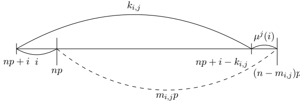
Figure 6.1: Schematic representation of the definition of m_{i,j}
