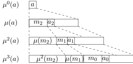
Figure 1.2: An illustration of what it means for a sequence ((m_i, a_i))_{0 \leq i \leq 2} to be a -admissible with respect to a substitution \mu .
