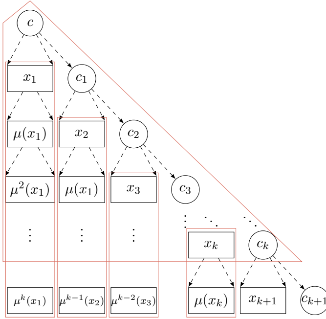
Figure 7.6: In the proof of Lemma 7.25, given a letter c , we inductively define \mu(c) = x_1 c_1 and \mu(c_i) = x_{i+1} c_{i+1} for every i \geq 1 , where x_i is a word and c_i is a letter for every i \geq 1 . We draw the tree \mathcal{T}_{\mu,c}^{\leq k+1} as defined in the proof of Lemma 7.25. Black rectangles correspond to words (note that we do not give information on the length here) and black circles to letters. The induction hypothesis tells us that, up to labeling, every color-framed subtree is equal to its corresponding subtree in \mathcal{T}_{\mu,d}^{\leq k+1} .
