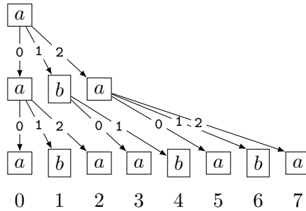
Figure 1.4: The first levels of the tree associated with the substitution \phi^2 .
