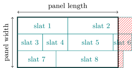
Figure 1: Toy example of assembly scheme to build one CLT panel in 2D
