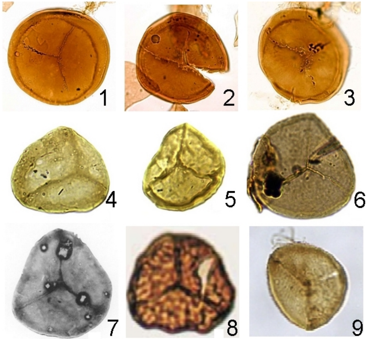
Comparison of miospores with true trilete marks (7–9) and pseudo-trilete marks (1–3), with Late Ordovician trilete spores from Saudi Arabia (4–6). 1–3: Unpublished pictures from P. Breuer, Lower to Middle Devonian, Saudi Arabia: Gneudnaspora divellomedia var. divellomedia (Chibrikova) Breuer et al. , 2007 showing pseudo-trilete marks. 4–6: Pictures from Wellman et al. (2015): they are the Late Ordovician trilete spores from Saudi Arabia, which are considered as doubtful by some authors. 4: Ambitisporites avitus Hoffmeister, 1959 sensu Steemans et al. (1996) with a true trilete mark. 5: Chelinospora prisca Wellman et al. , 2015 with a true trilete mark, encroachment of the curvaturae is well visible. 6: Aneurospora sp. A in Wellman et al. (2015) with a thin, straight, regular, trilete mark reaching the curvaturae. 7–9: Copy examples of published true trilete spores from the Silurian up to Lochkovian. 7: Ambitisporites avitus Hoffmeister, 1959 (extracted from Hoffmeister, 1959: pl. 1, fig. 10). 8: Chelinospora retorrida Turnau, 1996 (extracted from Filipiak et al. , 2012: fig. 4F). 9: Aneurospora extensa (Naumova) Turnau, 1996 (extracted from Turnau & Markiewicz, 2010: pl. 1, fig. 3).
