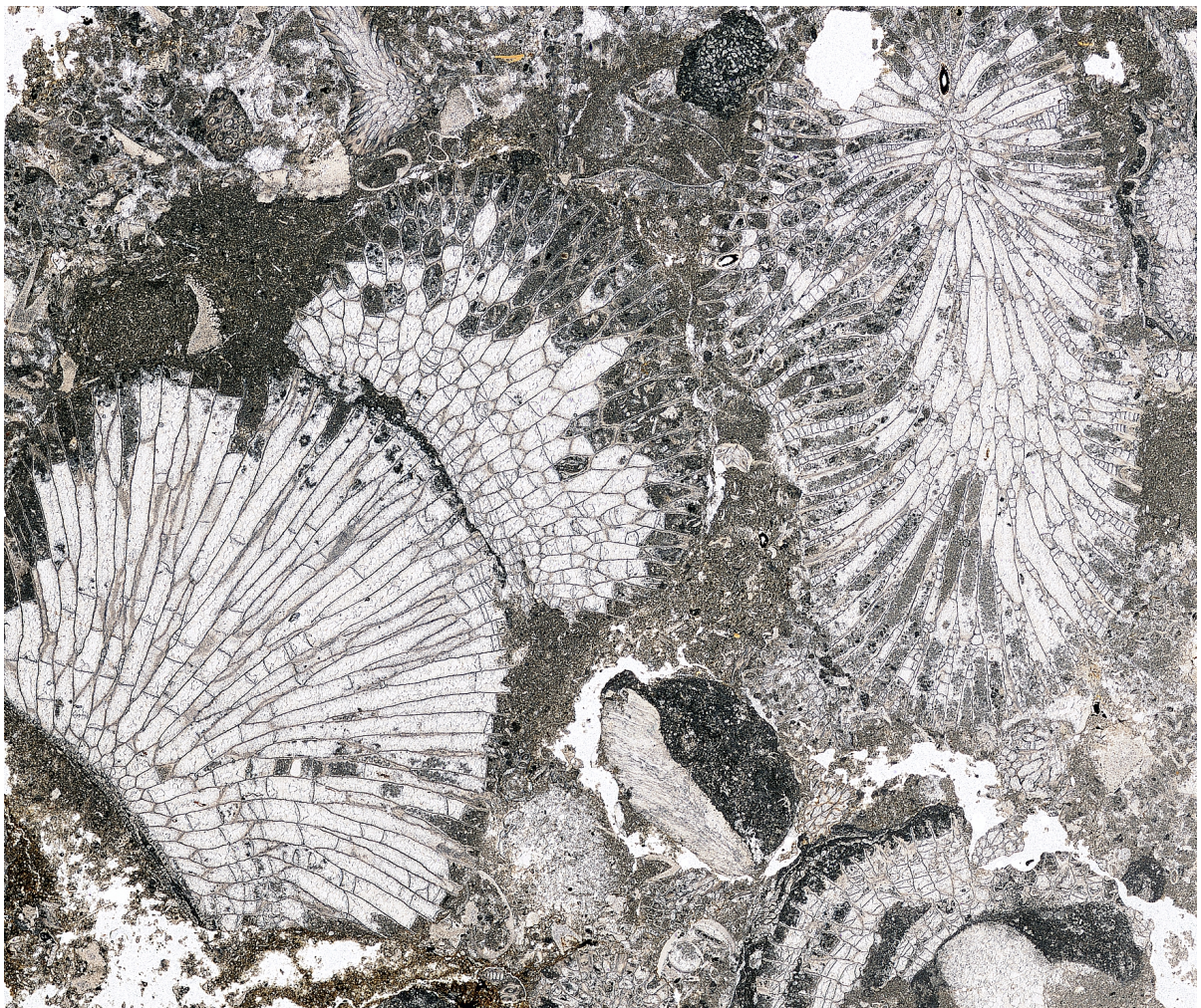
Thin section from the Vasalemma Quarry (Katian), Estonia, containing bryozoans and other fossils (©Andrej Ernst).
