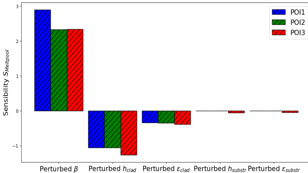
Fig. 10. Sensitivity of the melt pool depth for the 2D model. From [1].
