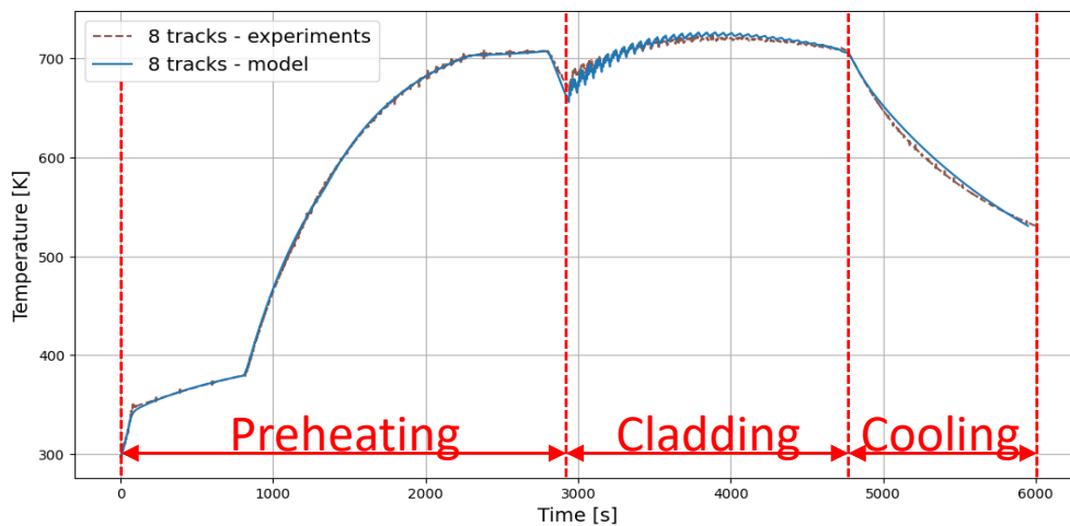
Fig. 3. Predicted and measured temperature curves for the thermocouple T 4 for the printing of an 8 tracks specimen.
