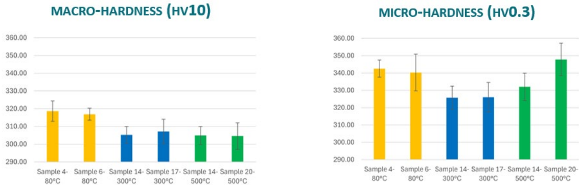
Fig. 5. Overview of hardness as obtained on the full-dense cubes after printing at various preheating temperatures that shows a decreasing trend for the macro hardness with increasing preheating temperature, and a U-shape trend for micro hardness; a) Macro hardness at 10 kg; b) micro hardness at 0.3 kg.
