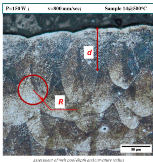
Fig. 6. Overview of the method used to assess both d , the depth of the MP (on the top layer), and the average curvature radius R .
