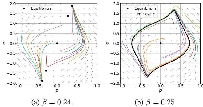
Fig. 2: Phase portraits for two value of \beta and \gamma = 0.2 . The system passes from 5 equilibria for \beta = 0.24 to 1 equilibrium with a stable limit cycle for \beta = 0.25 .
