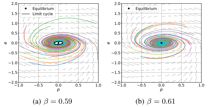
Fig. 3: Phase portraits for two value of \beta and \gamma = 0.2 . The stable limit cycle for \beta = 0.59 collapses into an equilibrium at \beta = 0.61 illustrating the Hopf bifurcation of Figure 1.
