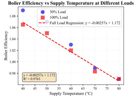
Fig. D.17. Boiler efficiency versus supply temperature at 30% and 100% load conditions. Scatter points show experimental measurements, with the dashed line representing the linear regression for full-load operation. The regression equation and R^2 value are provided in the figure.
