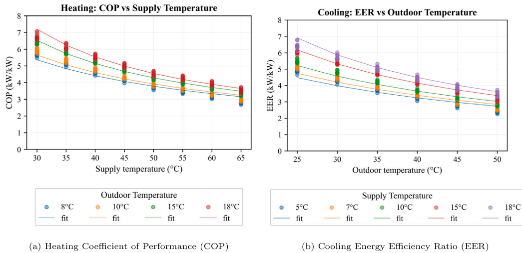
Fig. D.16. Measured and fitted performance curves for a reversible heat pump. Scattered points represent manufacturer data, while solid lines show the fitted model. Fitting was performed using nonlinear least-squares optimization on manufacturer data across varying supply and outdoor temperatures.
