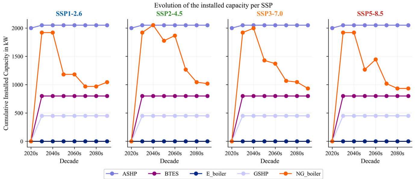
Fig. 7. Installed capacities as a function of time and SSP. Power values are reported in equivalent thermal power at the nominal operating point ( T_{\text{out}} = 7^\circ\text{C} , T_{\text{supply}}^h = 35^\circ\text{C} ).
