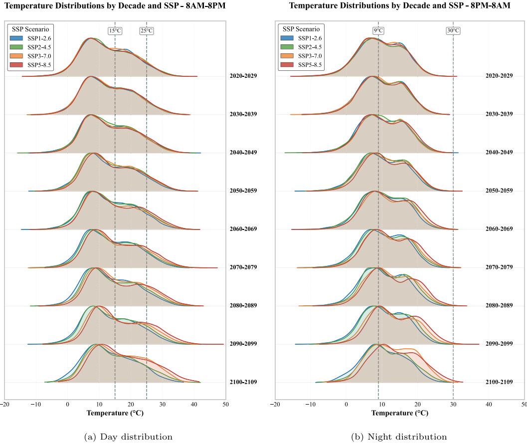
Fig. 3. Distribution of the daily-averaged temperature forecast for different decades and ssp. The vertical line indicates the bounds of the indoor comfort interval.
