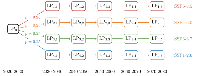
Fig. 1. A representation of our problem: each stage represents a decade, and each branch represents a different SSP impacting ambient temperatures and carbon prices evolution. The uncertainty lies between stages 0 and 1, as an SSP is sampled with probability 0.25. Afterwards, each SSP is modelled using the usual deterministic multi-stage modelling.
