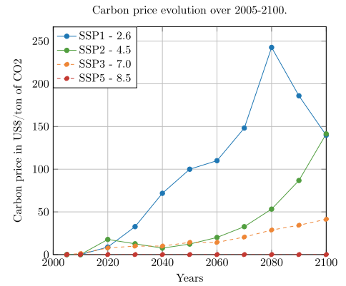
Fig. C.14. Carbon price evolution over the century depending on the SSP, adapted from Riahi et al. [58]. The carbon price for SSP3-7.0 was derived by taking half of the carbon price for SSP3-6.0 from Riahi et al. [58], and for SSP5-8.5, we take the carbon price would be zero.
