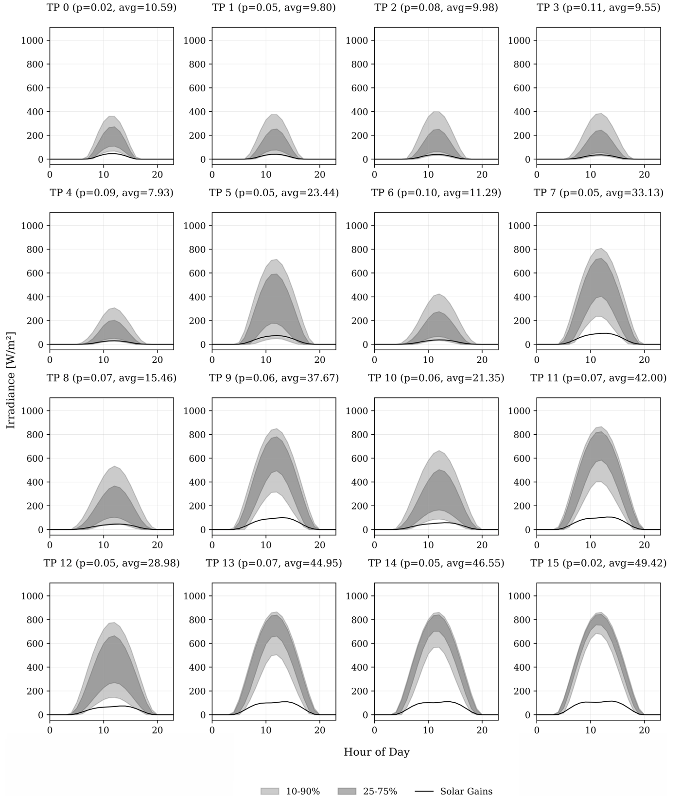
Fig. B.13. Representation of the solar gains per square meter of glass, compared to the total irradiance on a horizontal surface per square meter. The gray bands represent the distribution of the irradiance values that are assumed to lead to the representative solar gains.
