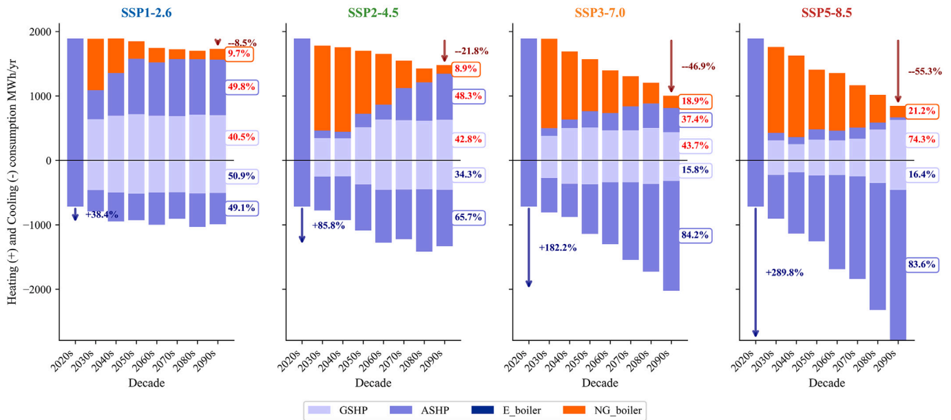
Fig. 8. Annual heating and cooling supplied by technology across SSPs and decades. Heating demand decreases as warming intensifies, while cooling grows from marginal to dominant in severe scenarios. Results for 2020 correspond to the initialised system, where heating and cooling are fully met by ASHP.
