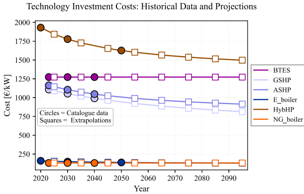
Fig. D.15. Technology investment cost trajectories. Circles denote historical data points from Prognos AG et al. [47]; squares indicate decadal extrapolations (2025–2095). Solid lines show fitted hyperbolic decay curves, capturing technology learning rates and asymptotic cost floors.
