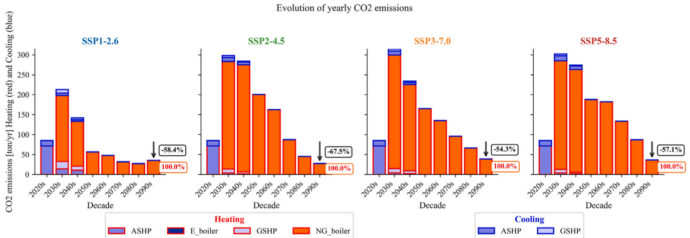
Fig. 10. Evolution of the carbon emissions across SSP and decades, decomposed based on their origin.
