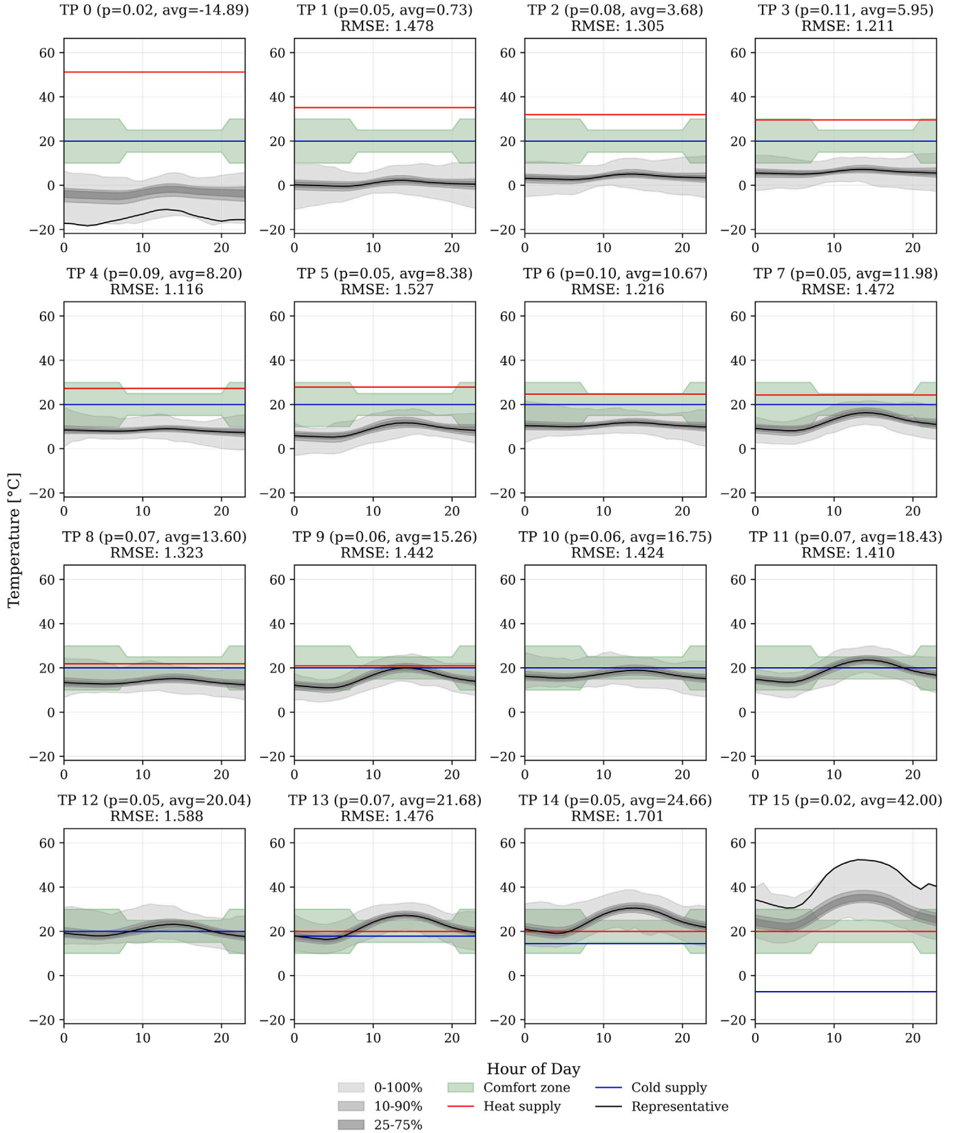
Fig. B.12. Representation of temperature for every typical day. The first and last typical days are represented by their most extreme scenarios to enhance the robustness of the system and avoid smoothing out (solid black lines). The gray bands represent the distribution of the temperature for the days effectively represented by the black curve. The red and blue lines represent the supply temperature for heating and cooling, respectively, under these conditions.
