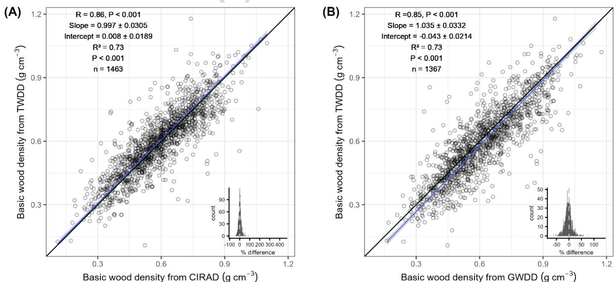
Figure 6 – Comparison of species-level basic wood density between Tervuren xyliarium Wood Density Database (TWDD) and other wood density datasets. The Major Axis (MA) regression line between the species-level average of the basic wood density from the Tervuren xyliarium Wood
