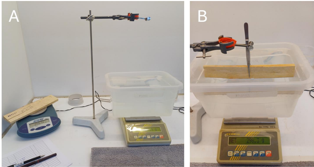
Figure 1 – Overview of methods to measure wood mass and volume for small wood samples. Set-up for wood density measurements of small samples. Mass is measured using a balance with a precision of 0.01g (A, on the left side). Volume is measured using the water displacement method by submerging the sample in a small water container with tweezers on a balance with a precision of 0.1g (B).
