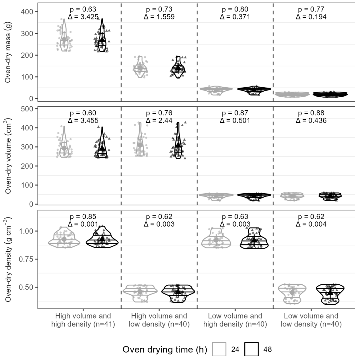
Figure 4 – Effect of oven-drying time on oven-dry mass, volume, and density for wood samples with varying volume and density in the Tervuren xyliarium. The rows represent the effect of drying wood for 24h (in grey) and 48h (in black) at 103°C on the oven-dry mass (top row, expressed in g), volume (middle row, expressed in cm 3 ), and density (bottom row, expressed in g cm -3 ). On the x-axis, the four categories based on the wood volume and density (high versus low) are shown. The sample size n is shown between brackets for each category. The violin plots show the probability distribution with the horizontal lines representing quantiles 25%, 50%, and 75%. The
