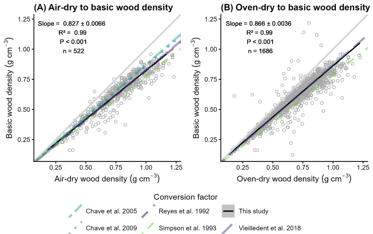
Figure 5 – Conversion factors to compute basic wood density from air- and oven-dry wood density for African tree species. (A) Relationship between air-dry (x axis) and basic bole wood density (y axis). (B) Relationship between oven-dry (x axis) and basic bole wood density (y axis). Dots represent individual wood density measurements for 1,686 samples across five sites in Central Africa, covering 191 tree species, 131 genera, and 41 families. Solid black lines show Major Axis (MA) regression lines, with the 95% confidence interval shown in grey. The slope of the MA regression (i.e., conversion factor), r-squared, P-value, and sample size (n) are shown in the upper left corner. Relationships from other studies are shown including Chave et al. 1 using the formula of Sallenave et al. 47 ( slope_{air}=0.872 at 12% moisture content; dotted line), Chave et al. 4 ( slope_{air}=0.86 at 12% moisture content; two dashed line), Vieilledent et al. 2 ( slope_{air} at 12% moisture content = 0.828, slope_{oven}=0.868 ; long dashed line), Reyes et al. 48 ( slope_{air}=0.821 ; dashed line), and Simpson et al. 46 ( slope_{air} at 12% moisture content = 0.778, slope_{oven}=0.785 ; dot dashed line) (see legend at bottom).
