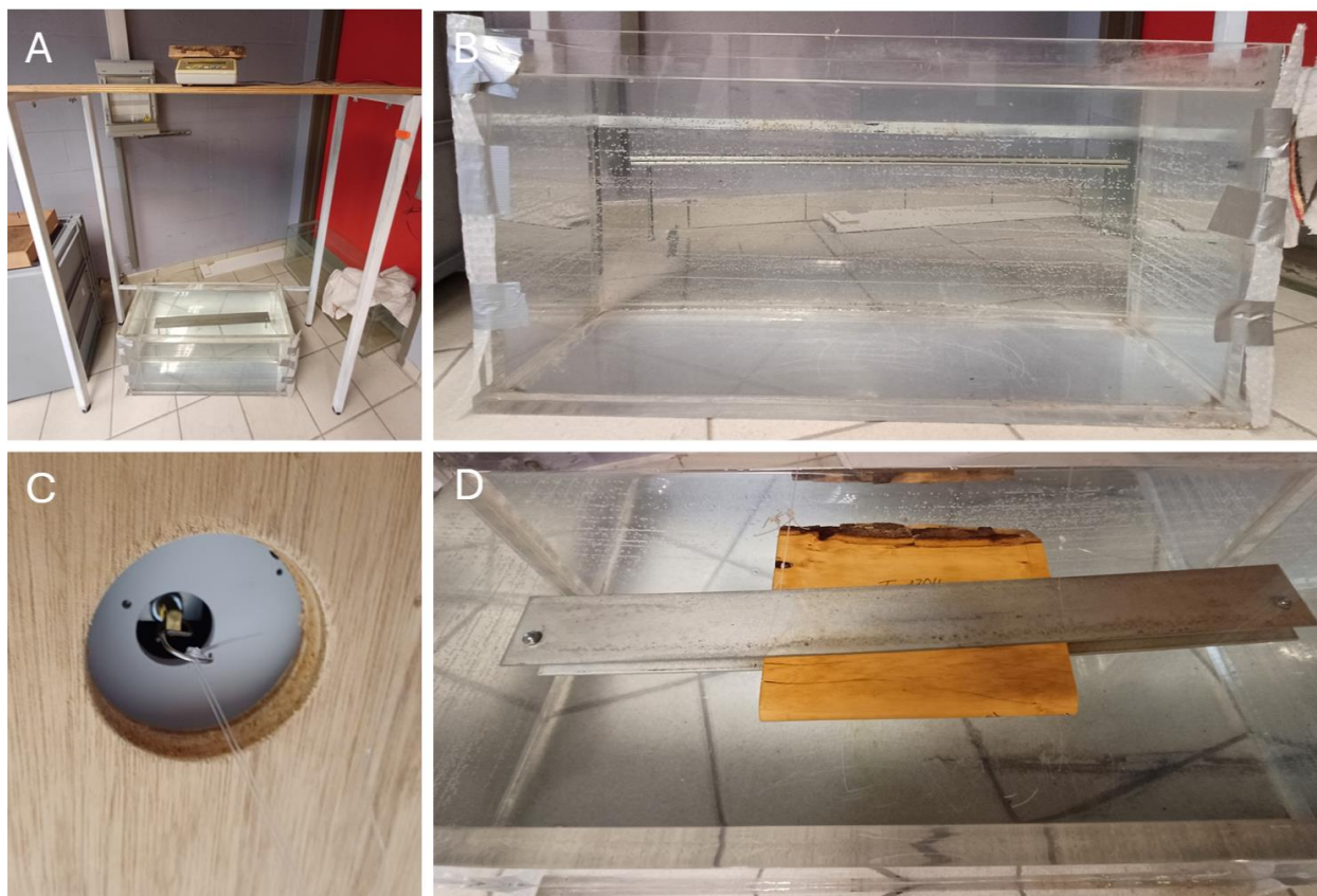
Figure 2 – Overview of methods to measure wood mass and volume for large samples. Set-up for wood density measurements of large samples (old samples in the collection) (A). Mass is measured using a precision balance of 0.1g (located on the shelf at the top of image A). Volume is measured by submerging the sample which is clamped between two metal plates in a large water container (B) attached to a balance with precision 0.1g using a plastic wire (C-D). The volume of the metal plates is subtracted from the total measured volume to calculate the volume of the wood.
