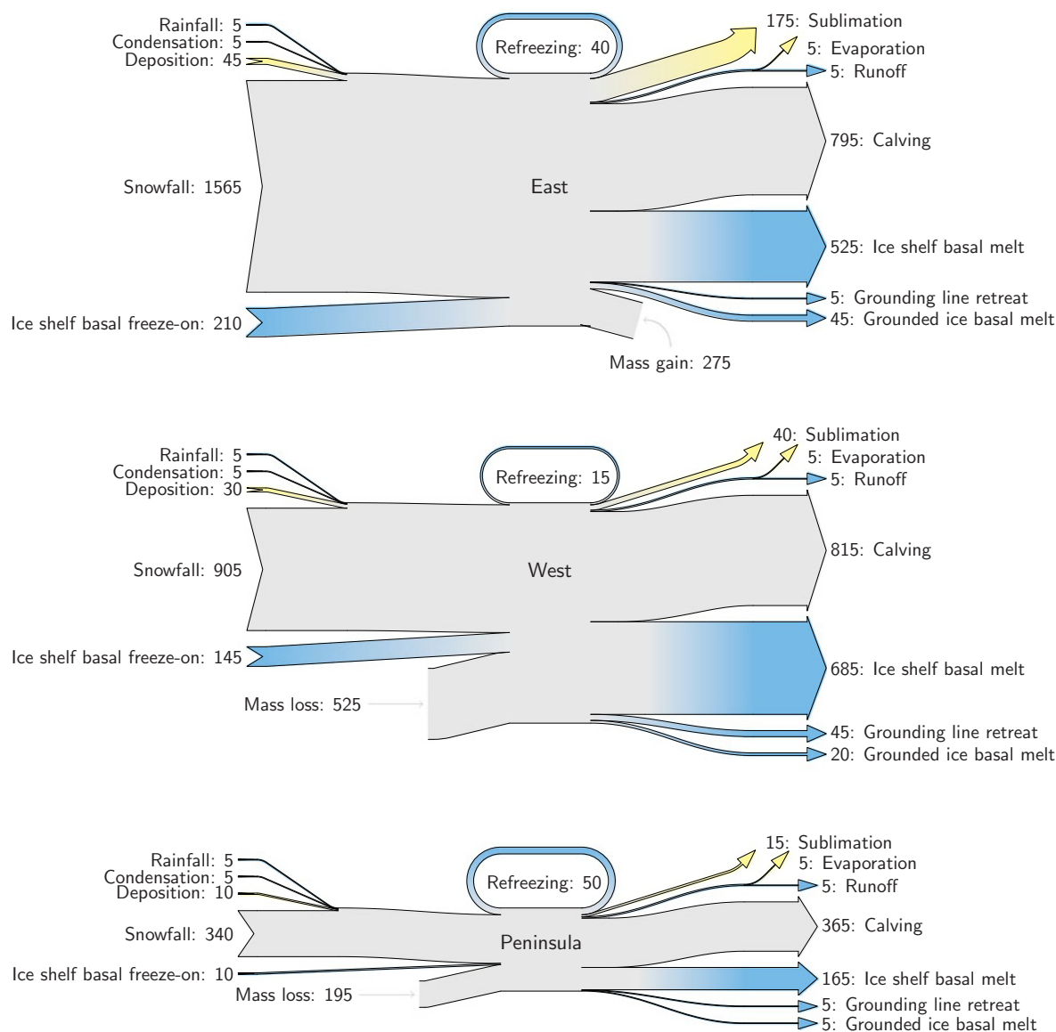
Figure 3. Sankey mass flow diagrams for three Antarctica regions: East, West, and Peninsula. Numbers are mass flow rate [ \text{Gt yr}^{-1} ]. All widths are proportional within and between images (and Figs 1 and 2). In East Antarctica mass gain is an output at the bottom that balances the diagram, because without it, there are more flows into the system than out of it.
