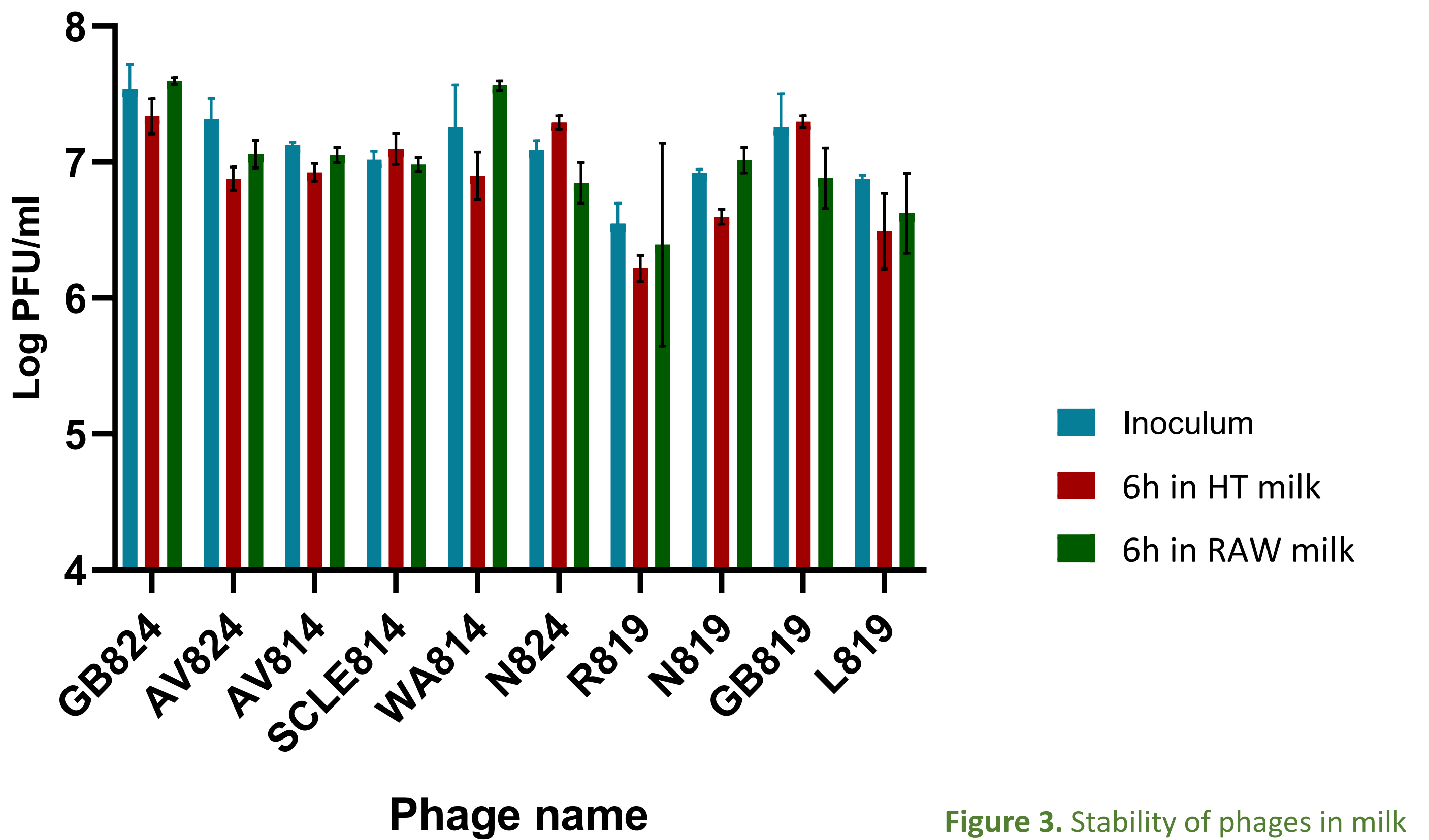
Figure 3. Stability of phages in milk
