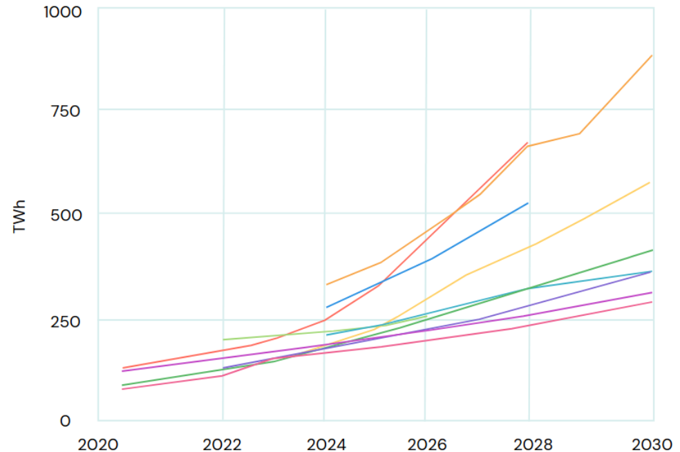
Data Centre Projected Yearly Energy Use (U.S.)
