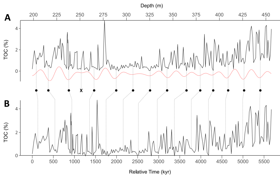
Fig. 5. Tuning of TOC using the 405-kyr LE cycle. A) Depth-domain TOC and bandpass filter output ( 1/30 to 1/15 \text{ m}^{-1} ) interpreted to reflect 405-kyr LE. B) Tuned, relative time-domain TOC. Dots reflect interpreted extrema in LE and are depth-time tie-points utilized to construct the age model. X reflects a potential additional extremum in LE which, after investigation, was not added for constructing the age model (see Suppl. Fig. S2).
