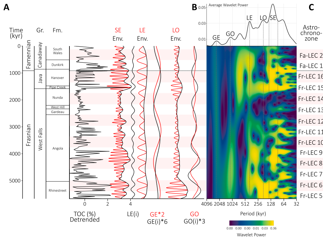
Fig. 6. Time-domain cyclostratigraphic analysis of TOC. A) WVC Stratigraphy: Stage, Group (Gr.) and Formation (Fm.), detrended TOC and bandpass filters corresponding to \sim 100 -kyr SE (red; 1/150 to 1/80 \text{ kyr}^{-1} ), its envelope (black), 405-kyr LE extracted from the envelope of SE (black; 1/505 to 1/305 \text{ kyr}^{-1} ), 405-kyr LE (red; 1/505 to 1/305 \text{ kyr}^{-1} ), its envelope (black), 2.4-Myr GE extracted from the envelope of GE (black; 1/2900 to 1900 \text{ kyr}^{-1} ), 2.4-Myr GE (red; 1/2900 to 1900 \text{ kyr}^{-1} ), 173-kyr LO (red; 1/203 to 1/143 \text{ kyr}^{-1} ), its envelope (black), 1.2-Myr GO extracted from the envelope of LO (black; 1/1500 to 1/900 \text{ kyr}^{-1} ) and 1.2-Myr LO (red; 1/1500 to 1/900 \text{ kyr}^{-1} ), respectively. B) Average and evolutive wavelet periodogram. Target periodicities (kyr) indicated by dashed vertical lines for GE (2.4 Myr), GO (1.2 Myr), LE (405 kyr), LO (173 kyr) and SE (95 and 131 kyr, respectively). C) Assigned astrochronozones (De Vleeschouwer et al., 2017; Whalen et al., 2017). The cone of influence was removed from the wavelet periodogram for visual clarity (see Suppl. A). Note relative time based on floating astrochronology. (For interpretation of the references to colour in this figure legend, the reader is referred to the web version of this article.)
