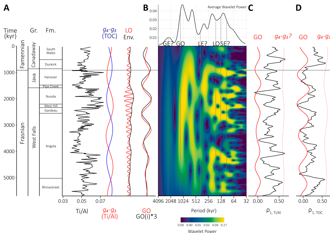
Fig. 7. Time-domain cyclostratigraphic analysis of sea-level change proxies. A) WVC stratigraphy: Stage, Group (Gr.) and Formation (Fm.), Ti/Al and bandpass filters corresponding to g_4-g_3 (Ti/Al, red; TOC GE, blue; 1/2900 to 1/1900 \text{kyr}^{-1} ), 173-kyr LO (red; 1/203 to 1/143 \text{kyr}^{-1} ), its envelope (black), 1.2-Myr GO extracted from the envelope of LO (black; 1/1500 to 1/900 \text{kyr}^{-1} ) and 1.2-Myr GO (red; 1/1500 to 1/900 \text{kyr}^{-1} ), respectively. Bandpass filter output corresponding to g_4-g_3 (TOC, Fig. 6) is added for comparison (blue). B) Average and evolutive wavelet periodogram of Ti/Al. Target periodicities (kyr) indicated by dashed vertical lines for GE (2.4 Myr), GO (1.2 Myr), LE (405 kyr), LO (173 kyr) and SE (95 and 131 kyr, respectively). C) \rho_1 , Ti/Al (black) and bandpass filter corresponding to 1.2-Myr GO (red) and g_4-g_3 (dotted red). D) \rho_1 , TOC (black) and bandpass filter corresponding to 1.2-Myr GO (red) and g_4-g_3 (dotted red). The cone of influence was removed from the wavelet periodogram for visual clarity (see Suppl. A). Note relative time based on floating astrochronology. (For interpretation of the references to colour in this figure legend, the reader is referred to the web version of this article.)
