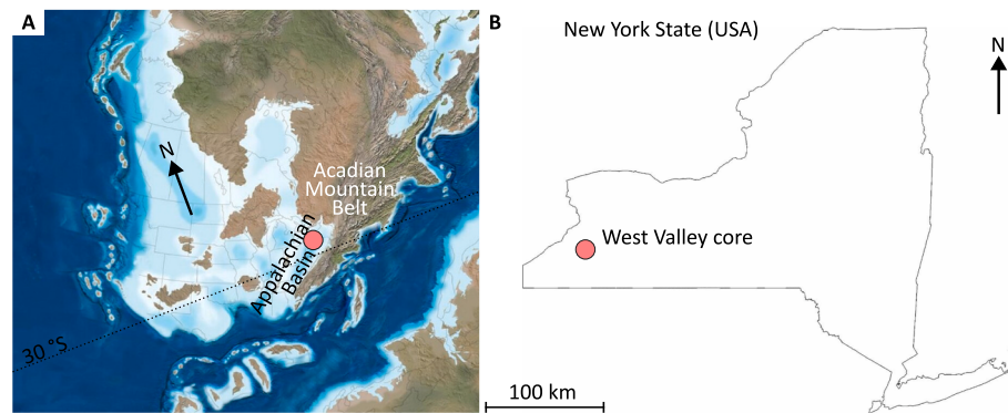
Fig. 1. Geological setting of the WVC. A) Late Devonian paleogeographic map (373 Ma) (courtesy of Ron Blakey, Colorado Plateau Geosystems). B) New York State (USA) modified from d-maps.com . WVC locality is indicated by a red dot. (For interpretation of the references to colour in this figure legend, the reader is referred to the web version of this article.)
