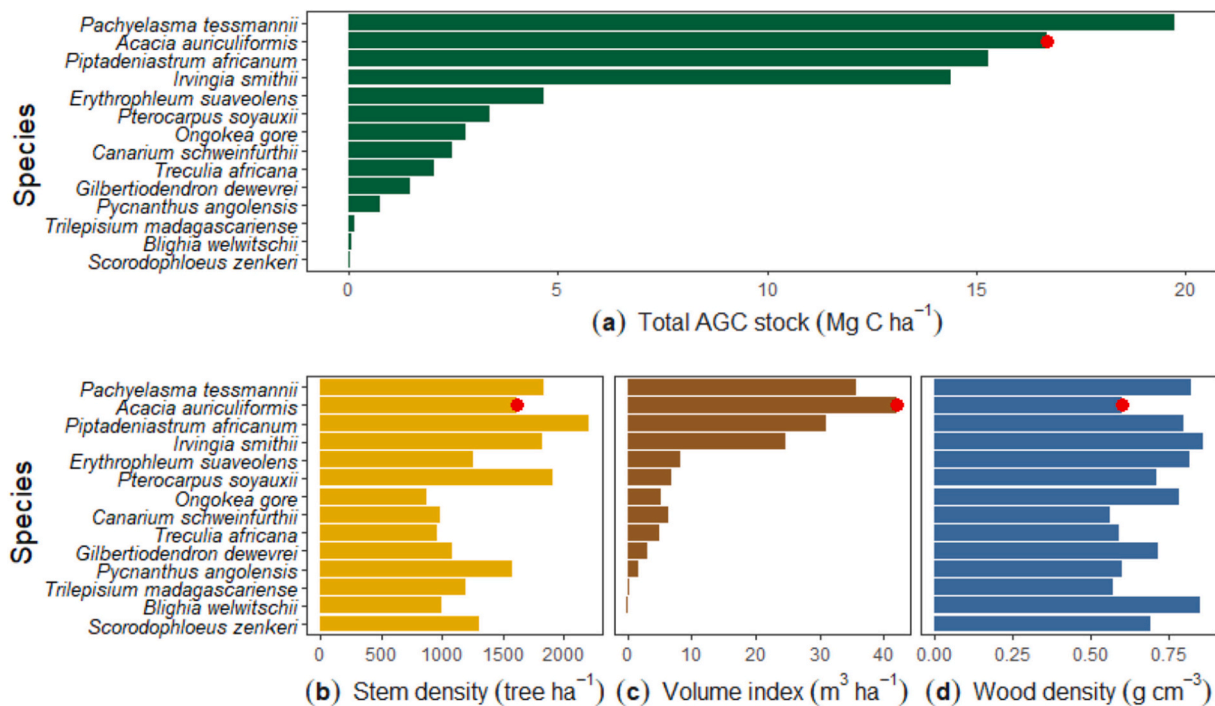
Fig. 4. Carbon sequestration and the related performance metrics for the studied tree species in 5-year-old plantations. (a) Total aboveground carbon stock (AGC, in \text{Mg C ha}^{-1} ), (b) Stem density (tree \text{ha}^{-1} ), (c) Total volume index (VI, in \text{m}^3 \text{ha}^{-1} ), and (d) Wood density (in \text{g cm}^{-3} ) extracted from the core samples using X-ray \mu\text{CT} scanning. The red dots on the graphs highlight the reference exotic species A. auriculiformis . (For interpretation of the references to colour in this figure legend, the reader is referred to the web version of this article.)
