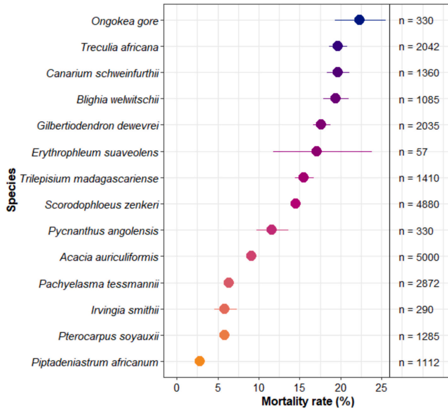
Fig. 2. Mortality rate of studied tree species from 5-year-old experimental plantations in Yangambi. The colour dots represent the estimated mortality rate ( \lambda ) over 5-years for each tree species presented on the y-axis. The horizontal lines extending from the dots represent the 95 % confidence intervals for the mortality rate ( \lambda ). The total number of initially planted seedlings per species is shown alongside the mortality rate on the right side of the graph. Species with the best survival performance are located toward the bottom of the graph. The graph does not show species with a 100 % mortality rate for visibility reasons.
