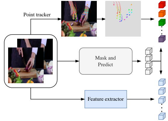
Figure 1. TrackMAE improves masked video modeling by jointly predicting spatial features and motion trajectories in a mask-and-predict fashion.
