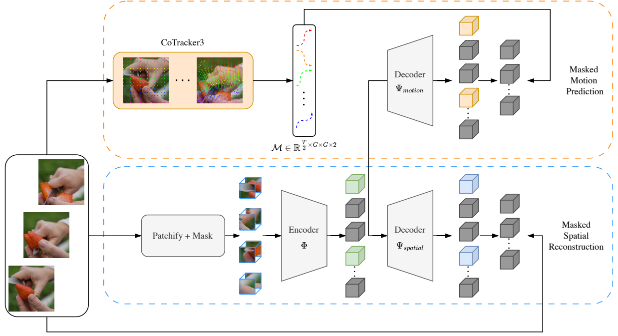
Figure 2. Overview of TrackMAE. In the lower branch, a video clip \mathbf{V} is first patchified and masked. The visible tokens are fed to a ViT encoder \Phi . Then the decoder \Psi_{\text{spatial}} aims to reconstruct spatial features based on the encoder output. In the upper branch, the input video clip is processed by a CoTracker3 module, extracting sparse point trajectories. The encoder output is then passed to a second decoder \Psi_{\text{motion}} , which aims to predict the extracted trajectories. The training objective combines both motion and spatial reconstruction.
