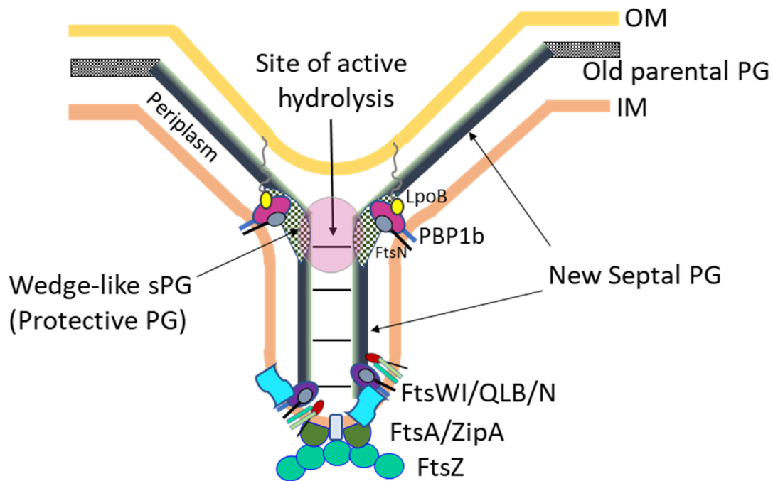
FIG 8 Model of E. coli cell division by septation-constriction. Model of the progression of septal PG synthesis and cell constriction depicting the respective role of PG synthase FtsW-FtsI and the class A PBP1b and their regulatory proteins. In this model, FtsW-FtsI drives septum synthesis inward at the leading edge, and PBP1b synthesizes a protective PG structure at the outer edge of the septum, where active hydrolysis and cell constriction take place that prevents cell lysis.
