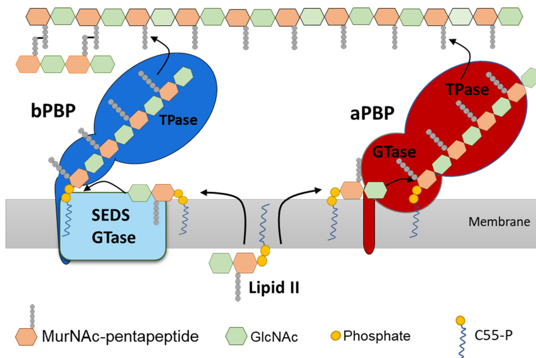
FIG 1 Overview of the final stages of PG polymerization. The PG precursor lipid II is assembled in the inner face of the cytoplasmic membrane and translocated to the outer face of the membrane by a flippase. Lipid II is then polymerized by the glycosyltransferase activities of the class A PBPs and SEDS and cross-linked to the preexisting PG sacculus by the TPase activities of aPBP and bPBPs.
