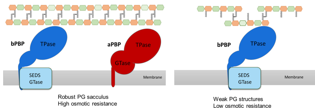
FIG 4 Correlation between PG structure and the PG synthases content. The presence of both SEDS-bPBP and aPBP provides the cell with a robust PG sacculus that can withstand high osmotic pressure. In the absence of aPBP, the PG structure is weaker, and the cells are unable to cope with high osmotic pressure, unless they are protected in an osmo-protective environment.
