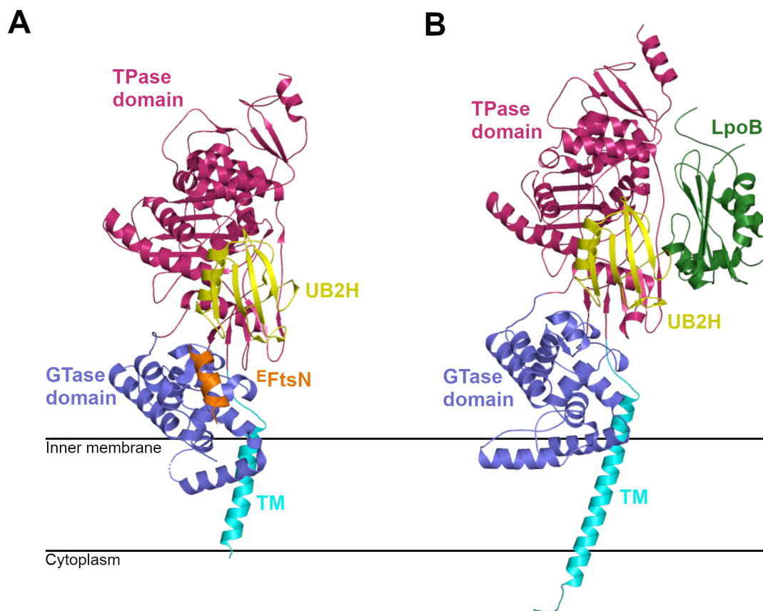
FIG 6 (A) Cartoon representation of the E. coli PBP1b structure in complex with the essential fragment of FtsN, F FtsN (PDB code 6YN0). (B) AlphaFold3 model of E. coli PBP1b in complex with LpoB (green cartoon). The quality of the model can be seen in the version of the figure colored according to the predicted local distance difference test (Fig. S1B).
