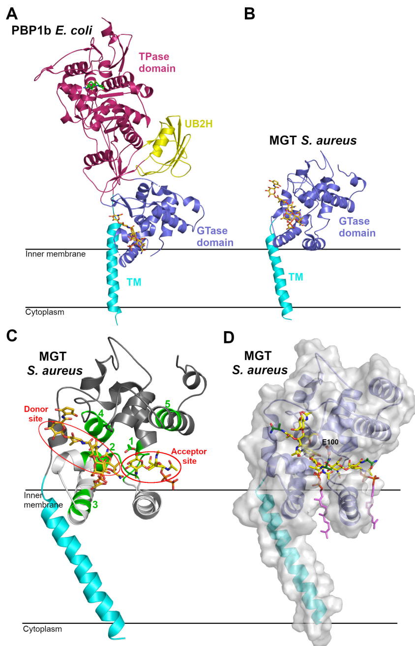
FIG 5 3D structures of PG polymerases from the GT51 family. (A) Cartoon representation of the Class A PBP1b from E. coli (PDB code 5HLA). (B) MGT from S. aureus (PDB code 3VMR). The GTase domain of both enzymes binds moenomycin (gold sticks), while the TPase domain of PBP1b is acylated by the cephalixin antibiotic (green sticks). (C) Same structure of MGT showing the five conserved motifs in green. The donor site binds moenomycin, and the acceptor site contains a lipid II analog from the superposed 3VMT structure. (D) AlphaFold3 model of MGT (gray surface and blue cartoon representations) in complex with a transition state analog made of a lipid II and a lipid IV molecule with 15 carbon long acyl chains (pink sticks) and the peptide moieties constituted of a single Ala (green sticks). The catalytic Glu100 is shown as blue sticks. The quality of the model can be seen in the version of the figure (Fig. S1A) colored according to the predicted local distance difference test. The details of the interactions between MGT and moenomycin, lipid II analog, and the transition state analog can be seen in Fig. S2A through C.
