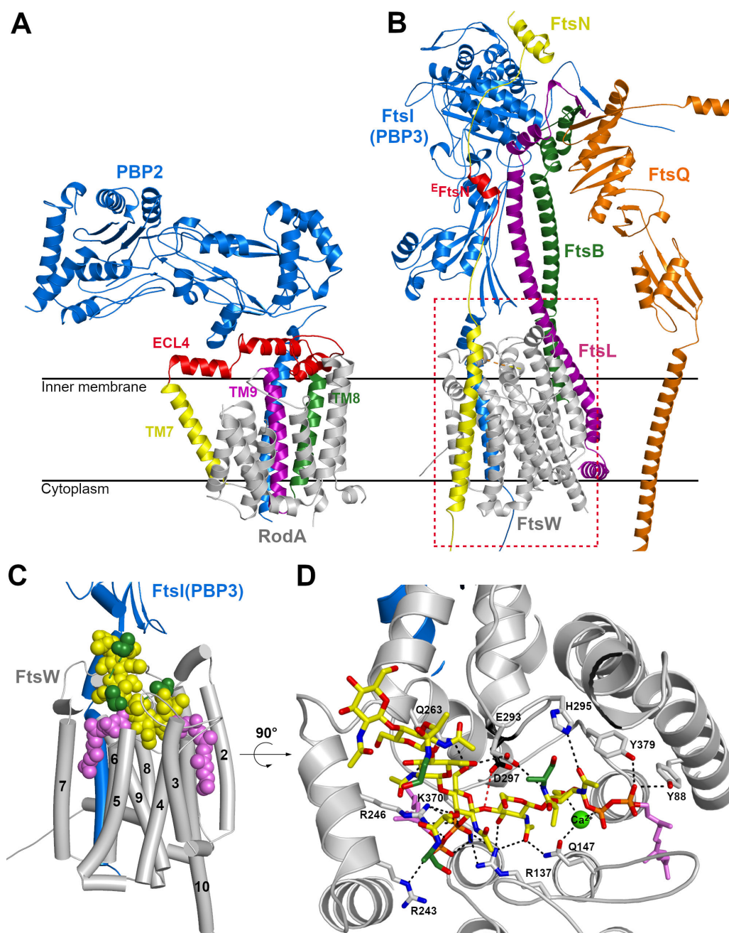
FIG 7 Structure and models of SEDS/PBP complexes. (A) Structure of the E. coli RodA/PBP2 complex (PDB code 8TJ3). (B) Cartoon representation of the AlphaFold3 model of the E. coli FtsBLQWIN complex. (C) AlphaFold3 model of the E. coli FtsWI complex (approximately corresponding to the red dashed rectangle in B) in the presence of a transition state analog made of a lipid II and a lipid IV molecule (glycan as yellow spheres) with 15 carbon long acyl chains (pink spheres) and peptide moieties constituted of a single Ala (green spheres). (D) Similar to C with a 90° rotation, the transition state analog is shown as sticks. Residues of FtsW making putative polar contact (dashed lines) are displayed as gray sticks except for the catalytic D297 in black. The putative Ca 2+ ion required for activity is shown as a green sphere. The quality of the models can be seen in the version of the figure colored according to the predicted local distance difference test (Fig. S1C and D).
