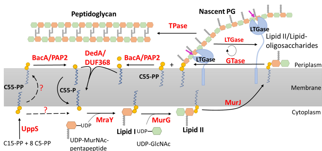
FIG 3 Overview of the undecaprenyl-phosphate lipid carrier (Upp-P or C55-P) cycle in the PG metabolism pathway. C55-PP is formed de novo by UppS and gets dephosphorylated by an unknown mechanism. The Upp-P is also recycled by the Up-PP phosphatases BacA and PAP2 and translocated to the cytoplasmic side of the membrane by DedA/DUF368 after Up-PP release during PG polymerization. Upp-P is used as a carrier of P-MurNAc-(pentapeptide)-GlcNAc added by MraY and MurG to form lipid II. The latter is translocated by the flippase MurJ to be polymerized by the GTases. The nascent glycan chain elongation is cleaved by specific PG hydrolases (MltG) that release a lipid-free glycan chain that is cross-linked to the existing PG sacculus by the TPases, whereas the lipid-linked oligosaccharide can be elongated again by the GTase.
