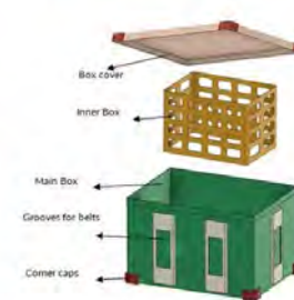
Fig.3: Simplified design of the Box
