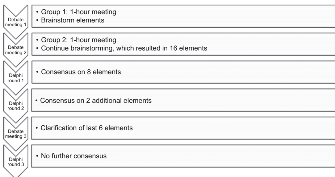
Figure 1: Delphi procedure.
