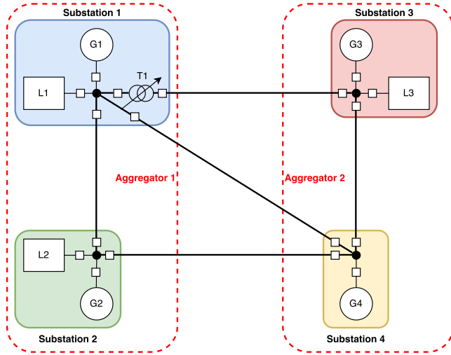
Fig. 2. Node-breaker view of the 4-bus test system.
