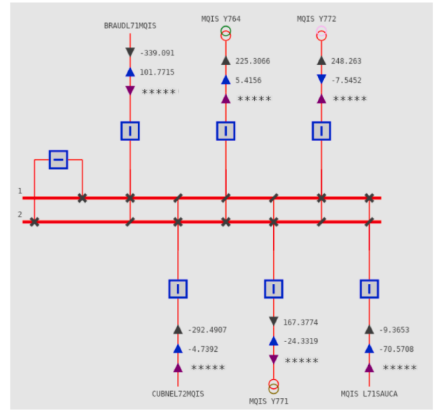
Fig. 6. Trainee view of the MQIS substation.
