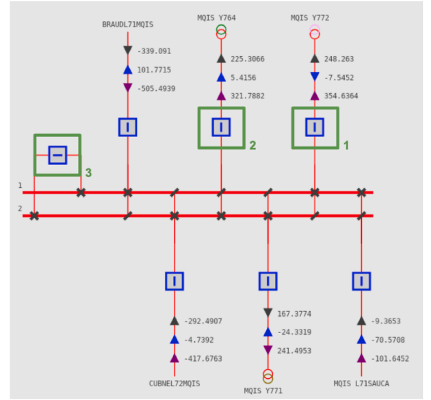
Fig. 5. Trainer view of the MQIS substation. From top to bottom, black arrows show active power values (in MW), blue arrows show reactive power values (in MVar), and purple arrows show current values (in A).
