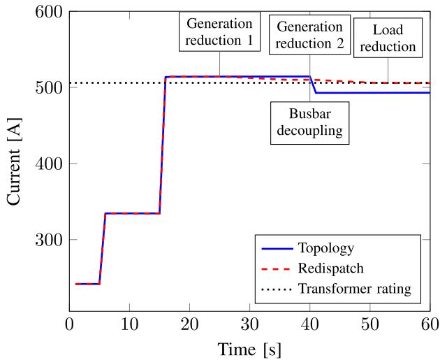
Fig. 7. Evolution of the current in the MQIS Y771 transformer in one scenario where the trainee opens the MQIS busbar coupler (full blue line), and in a scenario where the trainee performs generator and load reduction (dashed red line).
