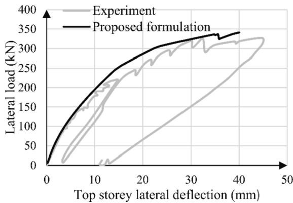
Fig. 14. Experimental and analytical load-deformation response Duong frame [45].
