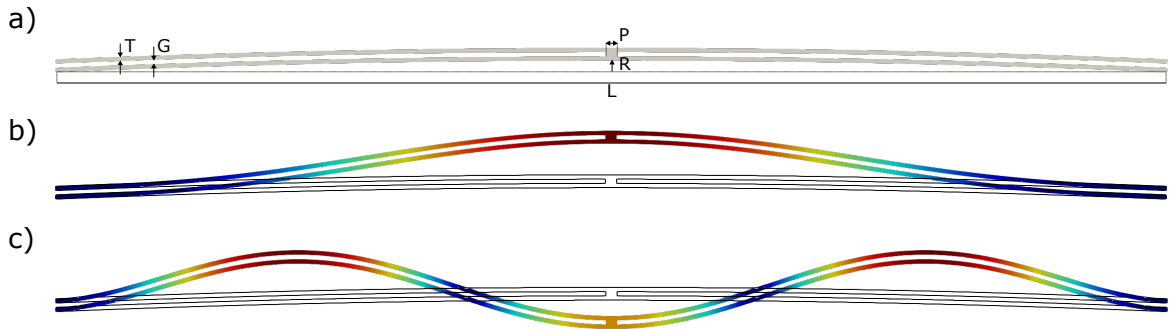
FIGURE 3 – (a) geometry of the internally resonant arch resonator. L = 649.5 \mu\text{m} , R = 6.675 \mu\text{m} , P = 6.5 \mu\text{m} , T = 2.5 \mu\text{m} , and G = 2.5 \mu\text{m} . (b) drive mode displacement field. (c) coupled mode displacement field. Blue colour is the zero of the scale, red is the maximum of the colour scale.
