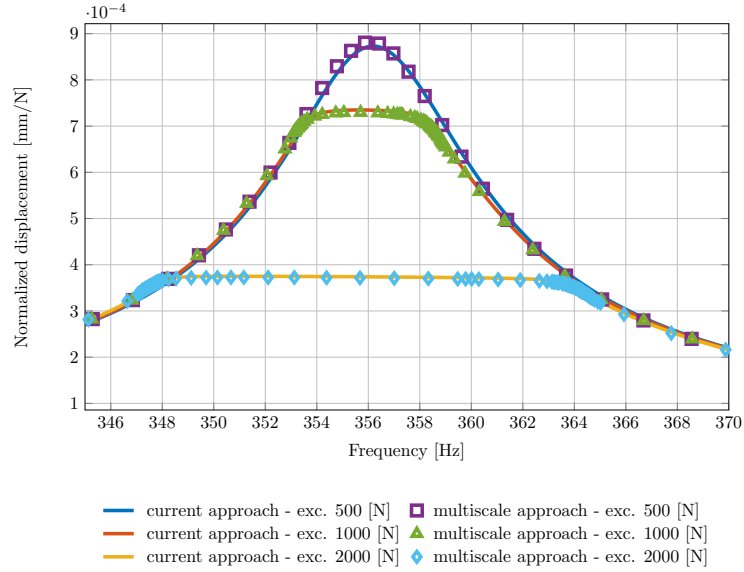
Figure 11: Frequency response functions of the resonator
