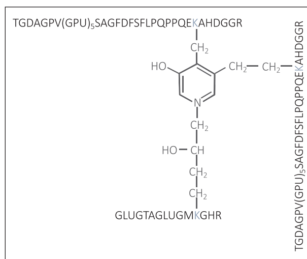
Figure 3. Molecular structure of ICTP in which the lysine residues in gray form a pyridinol crosslink. U stands for hydroxyproline.
