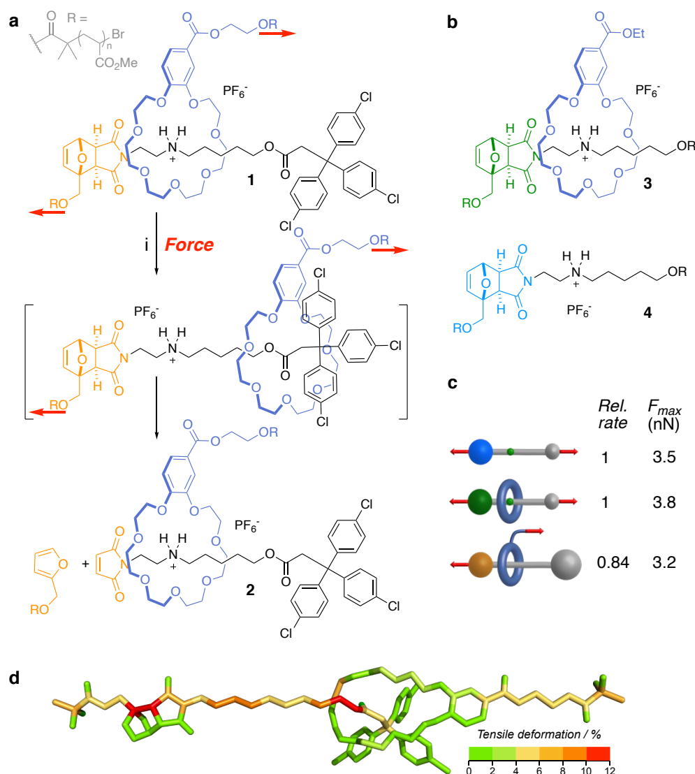
Figure 11. Rotaxane as a force actuator in a Diels Alder reaction. a) Mechanical activation of rotaxane 1. i) US (20 kHz, 13.0 W/cm 2 , 1 s ON/2 s OFF) THF, 5–10 °C, 240 min. Red arrows indicate direction of force. b) uncoupled rotaxane and linear mechanophore used as controls. c) relative rates of dissociation and maximum force before cleavage of mechanophores. d) distribution of tensile stress in rotaxane mechanophore obtained from CoGEF calculations (DFT B3LYP/6-31G*).
