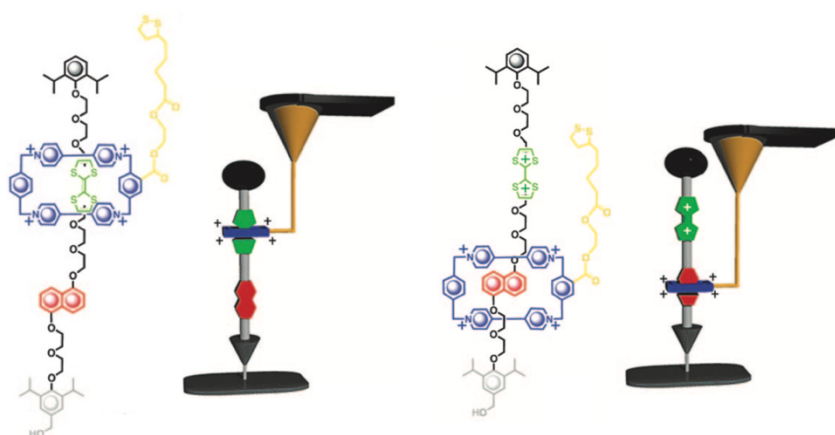
Figure 2. Chemical structure and schematic representation of the AFM force spectroscopy experiment of the bistable [2]rotaxane \text{R}^{4+} , in which an electron-poor cyclobis(paraquat- p -phenylene) ( \text{CBPQT}^{4+} ) ring is confined to an axis containing two electron-rich recognition sites, tetrathiafulvalene (TTF) and 1,5-dioxynaphthalene (DNP), by the presence of bulky 2,6-diisopropylphenyl ether stoppers at each end. The stopper close to the DNP site carries a hydroxymethyl group for subsequent attachment to silicon wafers. Left: The \text{CBPQT}^{4+} ring, which carries a very short tether terminated by a thioctic acid ester for attachment to a gold-coated AFM tip, displays a stronger interaction with TTF than with DNP and thus resides selectively on the former. Right: Chemical oxidation of TTF to \text{TTF}^{2+} results in a strong charge–charge repulsion between the \text{CBPQT}^{4+} ring and \text{TTF}^{2+} , a situation that causes the \text{CBPQT}^{4+} ring to shuttle to DNP in the oxidized [2]rotaxane \text{R}^{6+} . Adapted from ref.[31]
