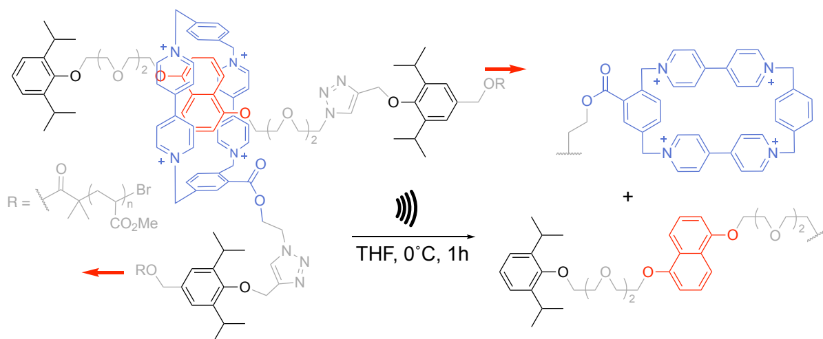
Figure 10. Mechanical activation of Stoddart's rotaxane in the centre of a poly(methyl acrylate) backbone, red arrows indicate direction of force, counter ions not shown for clarity
