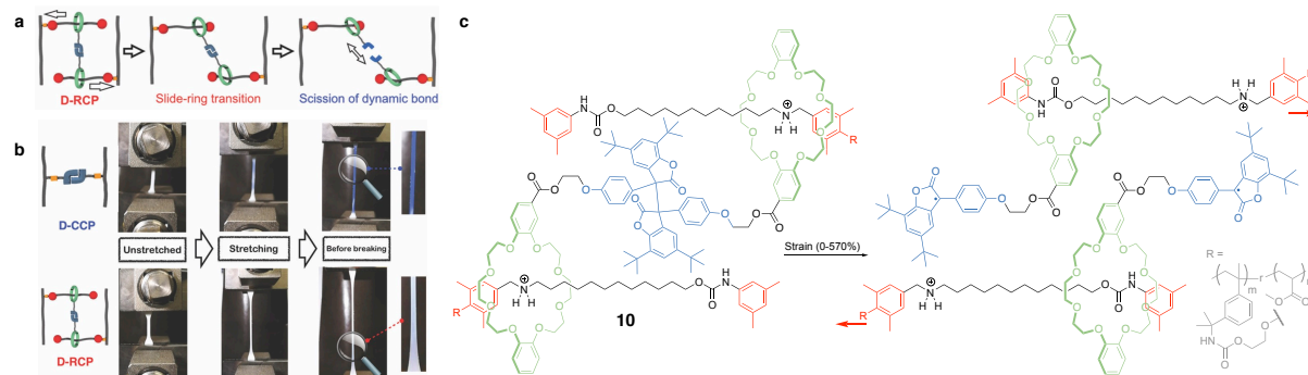
Figure 15. a) Schematic illustration of the activation of a rotaxane crosslinked polymer 10 . b) Photographs of polymers during tensile tests. c) Activation of rotaxane crosslinked polymer at 570 % elongation. Red arrows indicate direction of force. Adapted from ref. [68].
