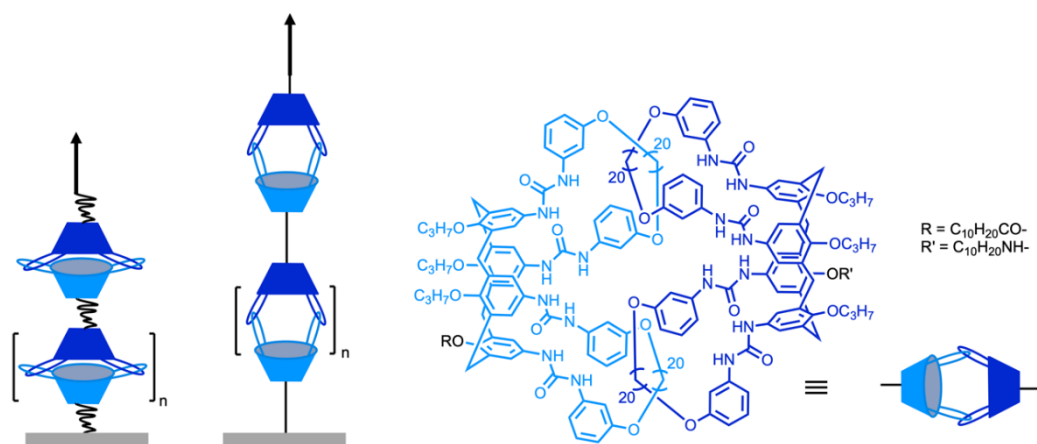
Figure 9. Left: Schematics of the AFM-based single-molecule force spectroscopy experiment of interlocked calix[4]arenes dimeric capsules. Right: Chemical structure of the capsules bound together by 16 hydrogen bonds.
