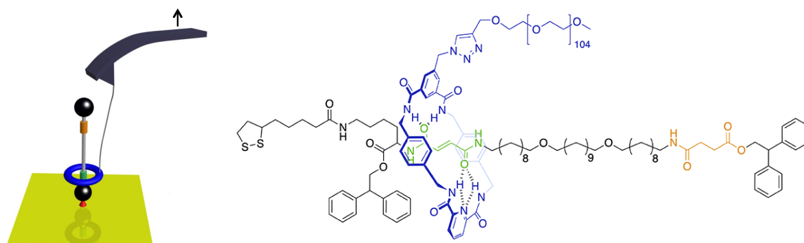
Figure 3. Left: Schematics of the single-molecule force spectroscopy experiment of the rotaxane. The rotaxane is grafted onto gold and the PEO tether is caught by the AFM tip. Right: Chemical structure of the rotaxane molecule. The rotaxane consists of a benzylic amide molecular ring (in blue) mechanically locked onto an axle by bulky diphenylethyl ester groups situated at either end. The axle bears a fumaramide group (in green) and a succinic amide-ester group (in orange), either of which can act as a binding site for the ring through up to four intercomponent hydrogen bonds. The affinity of the ring for the fumaramide site is much higher than for the succinic amide-ester site, so that the fumaramide:succinic amide-ester occupancy ratio is higher than 95:5. Next to the fumaramide binding site, a disulfide group (in red) was introduced to enable the grafting of the molecule onto gold substrates. A PEO tether (in blue) is attached to the ring in order to link the molecule to the AFM probe and track the motion of the ring along the axle. Adapted from ref.[25]
