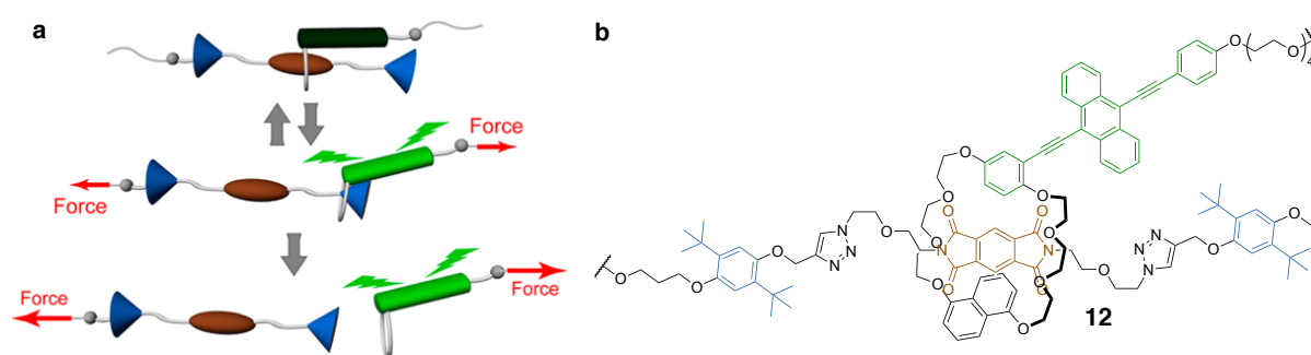
Figure 17. a) Schematic illustration of reversible and irreversible rotaxane mechanophores, red arrows indicate direction of force. b) Example structure of dual response rotaxane mechanophore 12 . Adapted from ref. [74].
