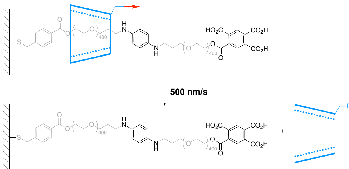
Figure 6. Single molecule force spectroscopy experiment of the deslipping behaviour of \alpha -CD over a tricarboxylic acid benzoyl stopper on a PEG track. The red arrow indicates direction of force.
