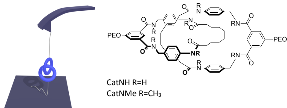
Figure 7. Left: Schematics of the single-molecule force spectroscopy experiment of the catenane. Right: Chemical structure of the [2]catenane of the benzylic amide family.
