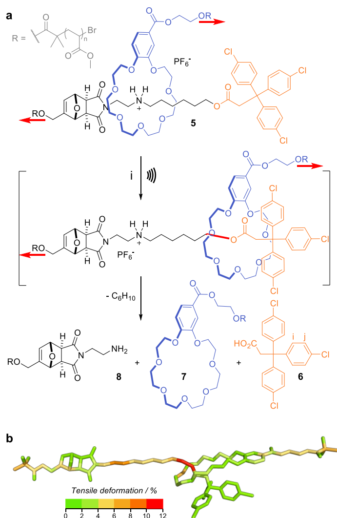
Figure 12. a) Mechanical dissociation of rotaxane mechanophore 5 by an unstoppering process. i) US (20 KHz, 11.5 W/cm 2 , 1 s ON/ 2 s OFF), CH 3 CN, 5-10 °C, 240 min. Red arrows indicate direction of force. b) distribution of tensile stress in rotaxane mechanophore obtained from CoGEF calculations (DFT B3LYP/6-31G*)
