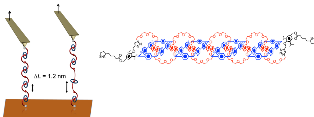
Figure 5. Left: Schematics of the single-molecule force spectroscopy experiment of the oligorotaxane. The theoretical variation of length after breaking one interaction between a free DNP and the contiguous ring is about 1.2 nm, on the basis of crystallographic data. Right: Chemical structure of the oligorotaxane molecule made of oligomeric dumbbells incorporating 1,5-dioxynaphthalene units encircled by cyclobis(paraquat-p-phenylene) rings.
