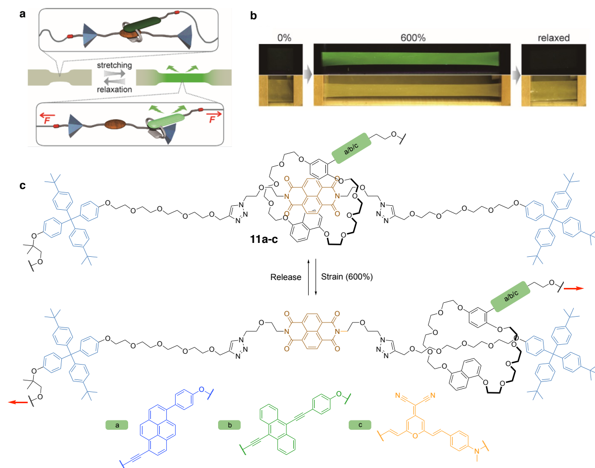
Figure 16. a) Schematic illustration of reversible rotaxane mechanophores 11a-c . b) Photographs of mechanophore-containing thin film during elongation. c) Activation of rotaxane mechanophores at 600 % elongation. Red arrows indicate direction of force. Adapted from ref. [72].
