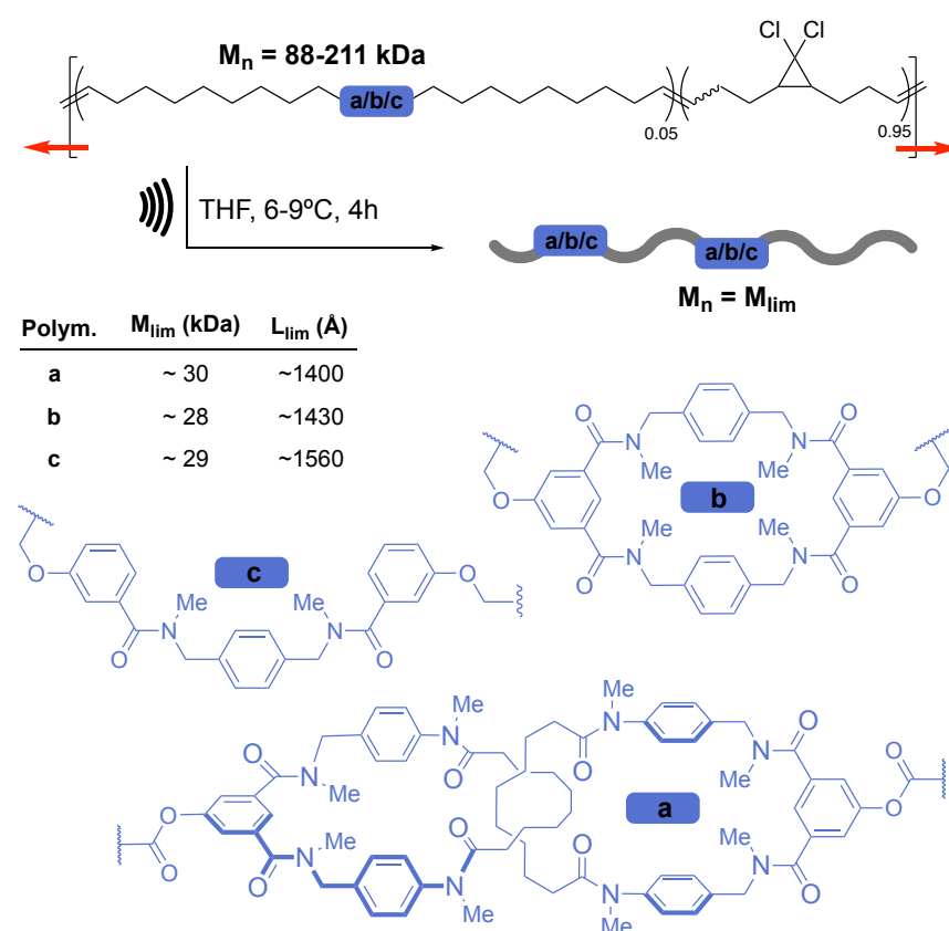
Figure 13. Sonication data for Craig's polymers. Limiting mass and length of polymers containing a catenane (a), compared to macrocyclic (b) and linear (c) controls. Red arrows indicate direction of force.
