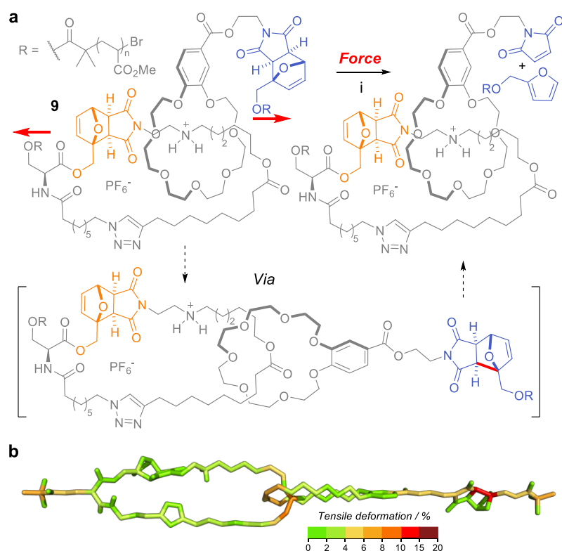
Figure 14. Mechanical activation of catenane mechanophore 9 . i) US (20 KHz, 13.0 W/cm 2 , 1 s ON/2 s OFF), CH 3 CN, 5-10 °C, 240 min. Red arrows indicate direction of force. b) Distribution of tensile stress in catenane mechanophore obtained from CoGEF calculations (DFT B3LYP/6-31G*)
