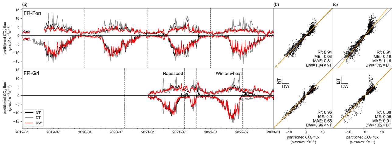
Fig. 12. (a) Daily averaged \text{CO}_2 partitioned fluxes. GPP and R_{\text{eco}} were calculated using commonly used night-time (NT, black) and day-time (DT, grey) partitioning methods and F^- and F^+ were calculated using wavelet-based direct DW-CS (DW, red) partitioning methods, all using DW-NEE as base data. Positive values show R_{\text{eco}} , and negative values show GPP. Dotted vertical lines show the start or end of the season (calendar years for forest site FR-Fon and cropping season for FR-Gri). (b) Daily NT versus DW GPP and R_{\text{eco}} (both on the same graph), in grey 1:1, in orange linear fit. On the bottom, statistics for GPP and R_{\text{eco}} combined the correlation coefficient ( R^2 ), the mean error (ME, \mu\text{mol m}^{-2} \text{s}^{-1} ), the mean absolute error (MAE, \mu\text{mol m}^{-2} \text{s}^{-1} ) and the linear fit. (c) same as (b) for DT versus DW comparison.
