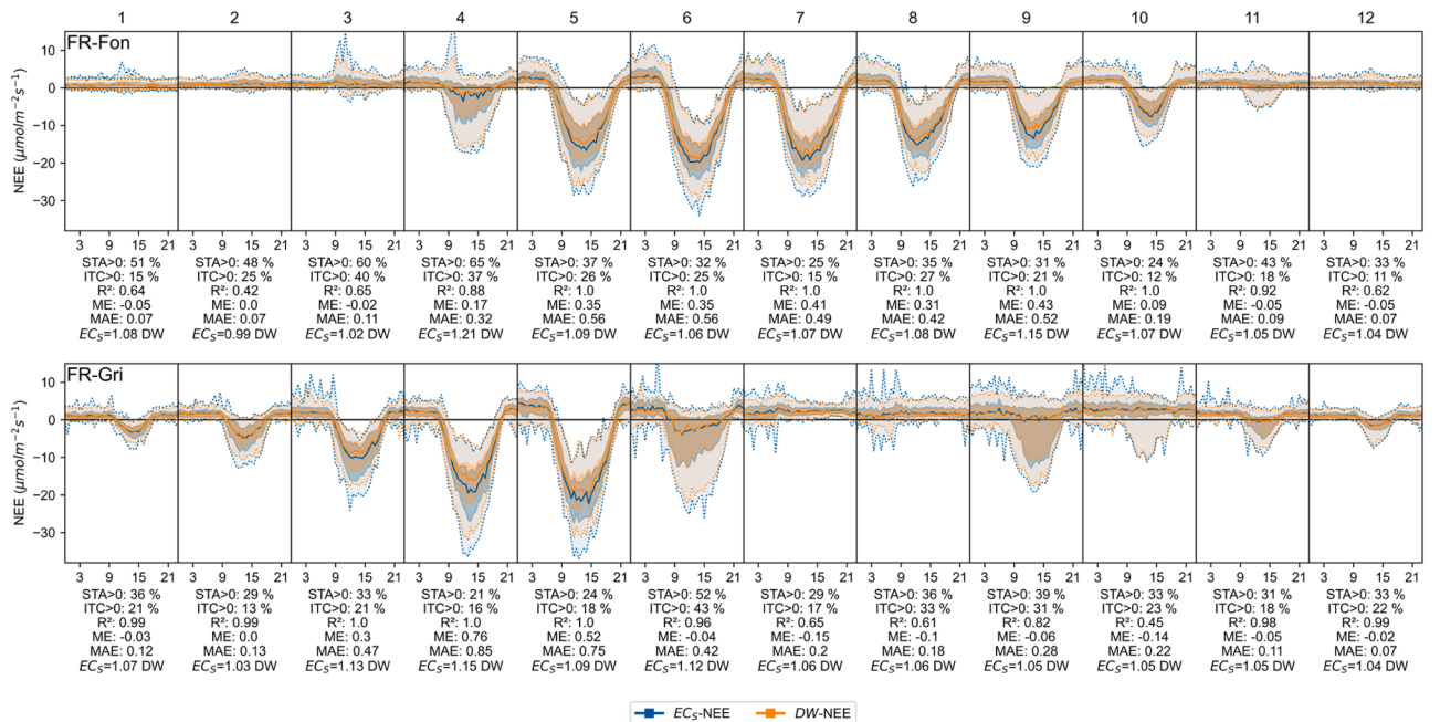
Fig. 7. Half-hourly NEE estimated monthly using EC_5 (blue) and DW (orange). The darker region indicates interquartile (25th and 75th percentile), and the lighter region with dotted lines indicates the 5th and 95th percentile. Below the curves, the monthly statistics are shown: the percentage of non-stationarity (STA>0) and low turbulence (ITC>0) data, the correlation coefficient ( R^2 ), the mean error (ME, \mu\text{mol m}^{-2} \text{s}^{-1} ), the mean absolute error (MAE, \mu\text{mol m}^{-2} \text{s}^{-1} ) and the linear fit.
