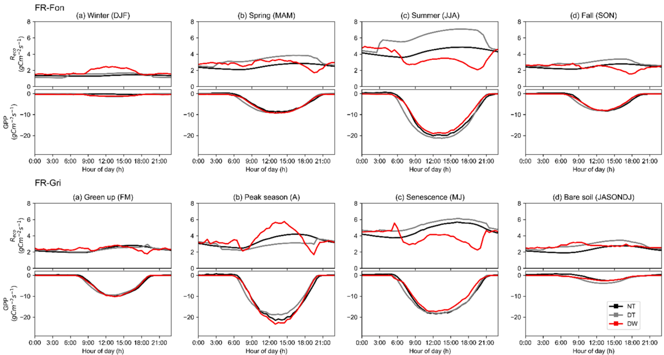
Fig. 13. Diel patterns of R_{\text{eco}} and GPP estimated calculated using commonly used night-time (NT, black), day-time (DT, grey) and wavelet-based direct DW-CS (DW, red) partitioning methods during climatic seasons (for FR-Fon) and the phenophases (for FR-Gri) of green-up, peak season, senescence, and bare soil (excluding September 2021 due to intermediate crop). Months are indicated by their first letter in parentheses. Note that R_{\text{eco}} and GPP are not on the same scale. Monthly results in .
