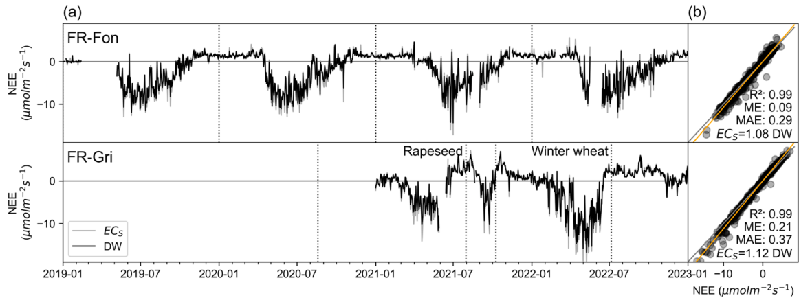
Fig. 6. Daily average \text{CO}_2 flux computed using wavelet-based (black, DW) and standard EC (grey, EC_5 ). Time series are shown in (a), while (b) shows ECs against DW-EC. The fluxes were not gap-filled.
