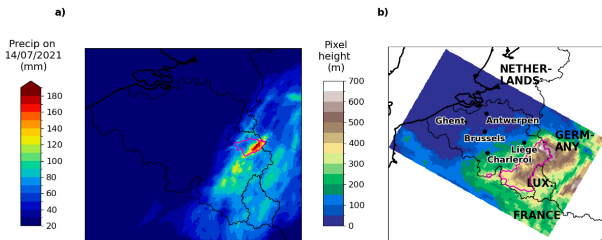
Fig. 1. (a) Precipitation on the 14th of July 2021 as recorded by the radar (Journée et al. 2021). The catchment of the Vesdre river is highlighted in purple. (b) MAR inner domain topography at 5 km. The Ardennian Massif is located in Belgium and highlighted in purple.
