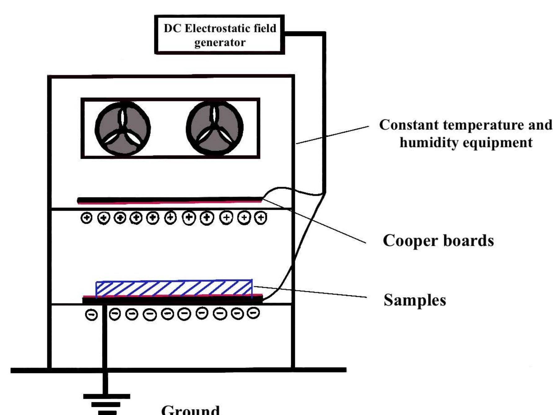
Figure 1. Equipment for Electrostatic Field Radiation and Temperature Control
