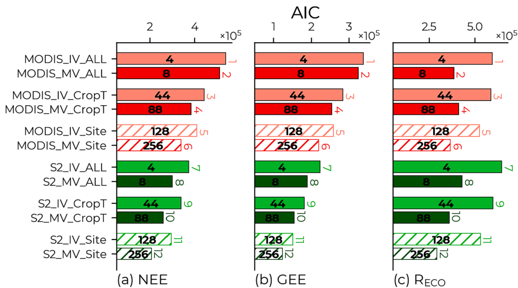
Fig. 4. AIC for the 12 scenarios calculated using half hourly data for (a) NEE, (b) GEE and (c) R_{\text{ECO}} . Hatched bars represent AIC of models where a distinct set of parameters was adjusted for each site-year. Numbers inside each bar correspond to the number of parameters optimized for each scenario while numbers above bars represent the scenario number (SN).
