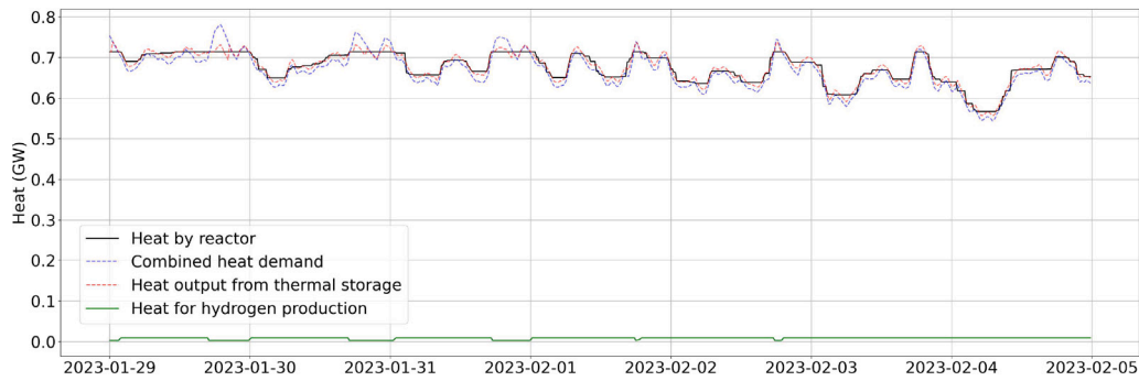
Fig. 7. Representation of heat management during a winter week (Configuration NH 3 -SOEC).
