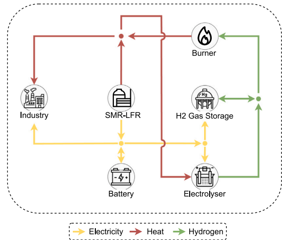
Fig. 4. Configuration 2 building upon Configuration 1 with the integration of a hydrogen production and storage system.
