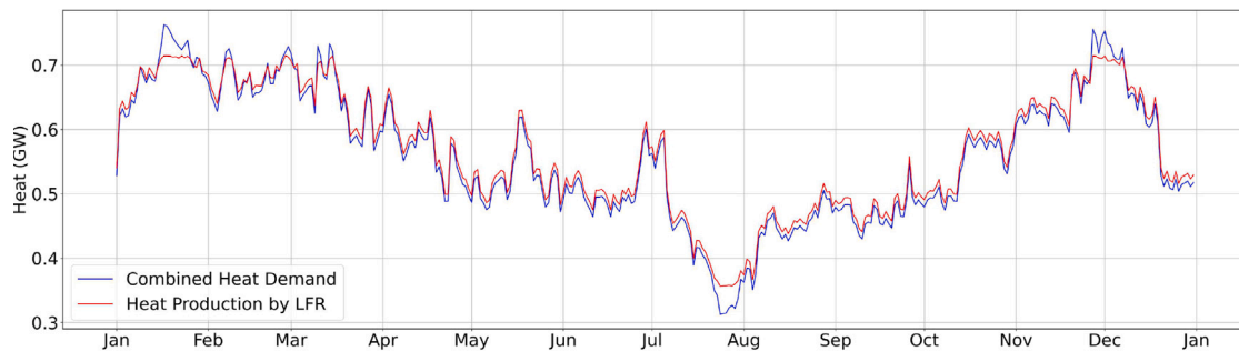
Fig. C.9. Representation of heat demand and the heat required for electricity demand, as well as the heat production of the reactor. Representation taken from model NH 3 -SOEC (similar to H 2 -SOEC).
