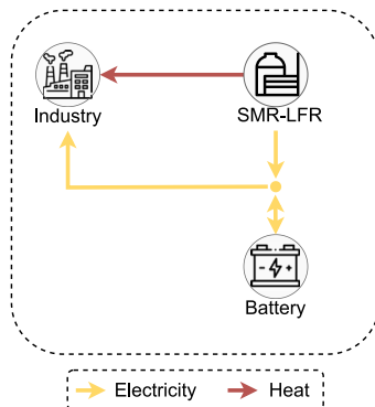
Fig. 3. Configuration 1 with LFR-SMR, industrial facility, and lithium-ion battery system.
