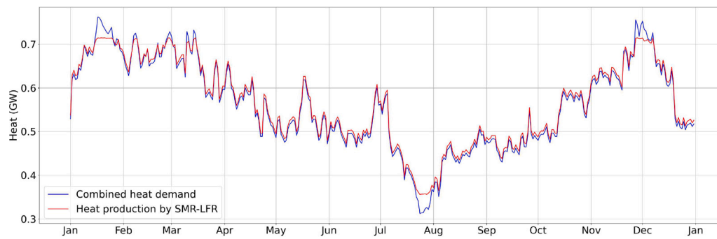
Fig. 6. Representation of heat demand and the heat required for electricity demand over a full year, as well as the annual heat production of the LFR-SMR. Representation taken from configuration H 2 -SOEC.
