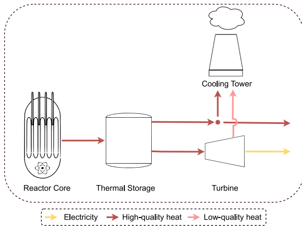
Fig. 2. Configuration of the LFR-SMR, including the reactor core, thermal storage, cooling tower, and the turbine. The energy system transforms the primary energy generated by the reactor core into two energy vectors: electricity and heat.
