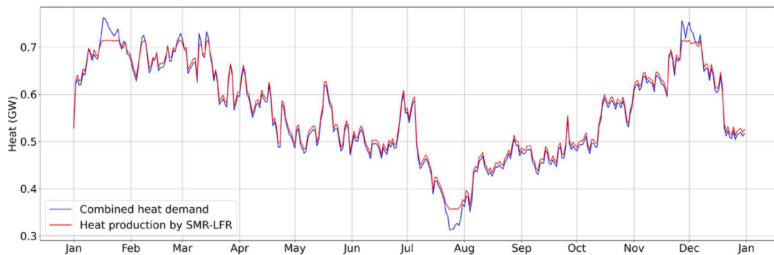
Fig. C.10. Representation of heat demand and the heat required for electricity demand, as well as the heat production of the reactor. Representation taken from model H 2 -AEC (similar to H 2 -PEM).
