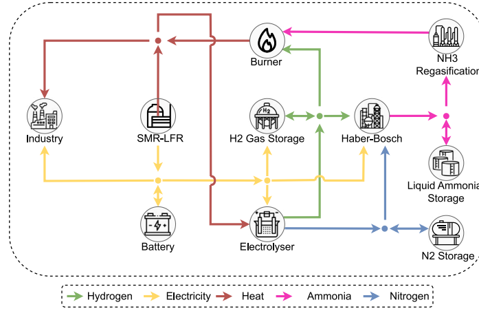
Fig. 5. Configuration 3 extending configuration 1 and 2, with the addition of an ammonia production and storage system.
