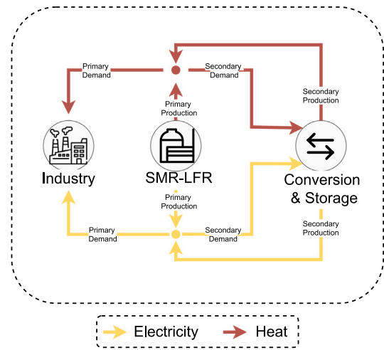
Fig. 1. Diagram of the primary and secondary demand and production flows.
