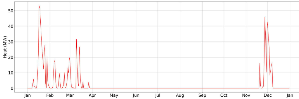
Fig. 8. Representation of heat production by the burner (Configuration H 2 -SOEC, similar to NH 3 -SOEC).
