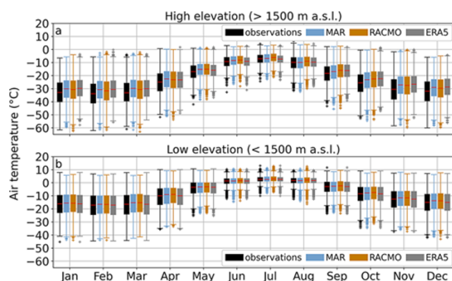
Figure 7. Boxplot of monthly 2 m air temperature from observations and models (MAR, RACMO and ERA5) at (a) high elevation sites and (b) low elevation sites. Median is shown with a red line, 1st and 3rd quartiles with a box, lower and upper whiskers with colored lines and outliers as a cross.
