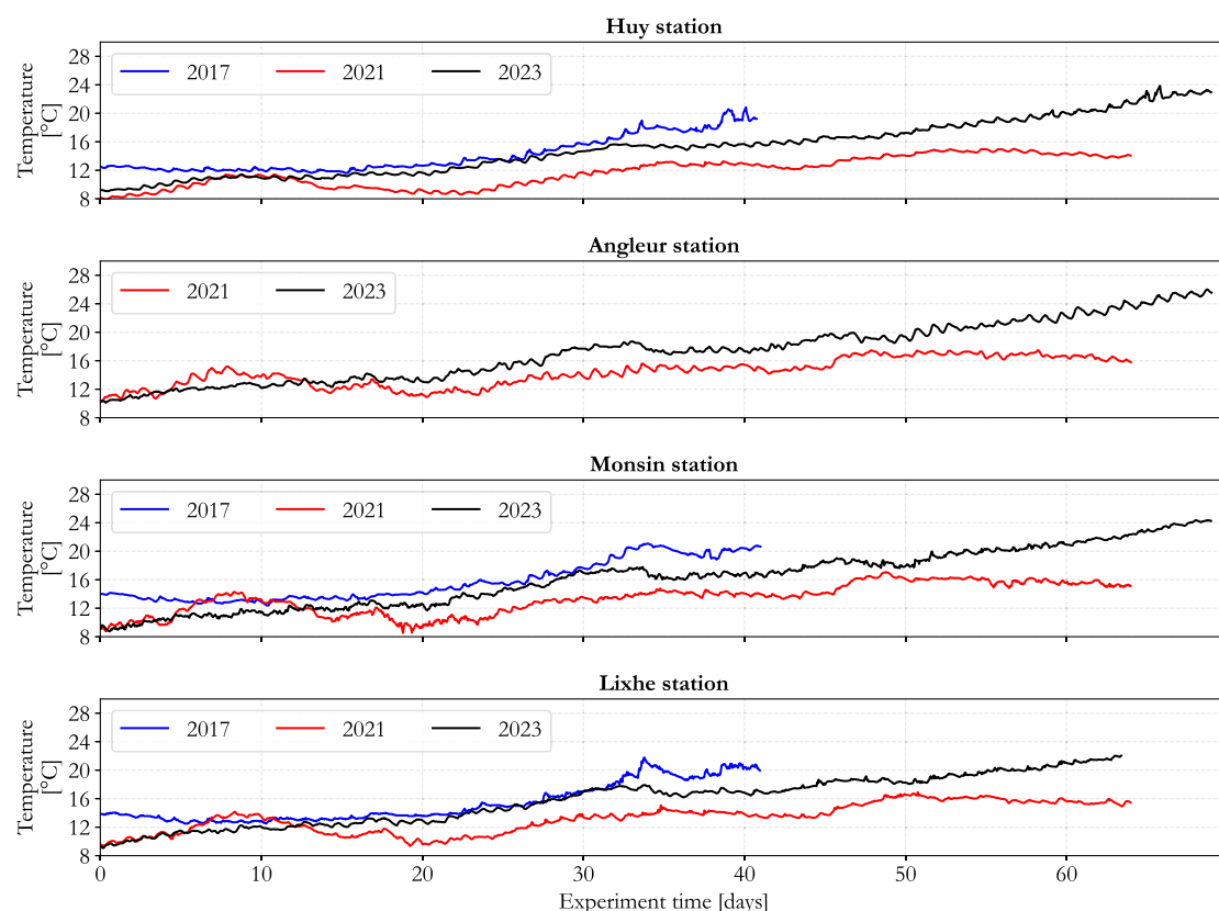
Fig. 4. Recorded water temperatures during the 3 experiments from upstream to downstream.
