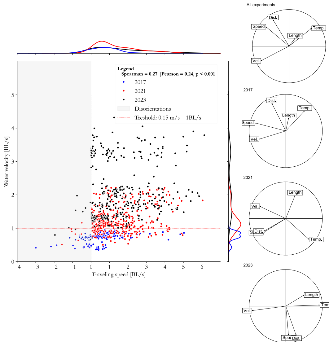
Fig. 6. Influence of water velocity on smolts traveling speed. Correlation circles explain the relationships between variables with Vel.: water velocity, Length: smolt length, Temp.: water temperature, Dist: distance already migrated by the smolt.
