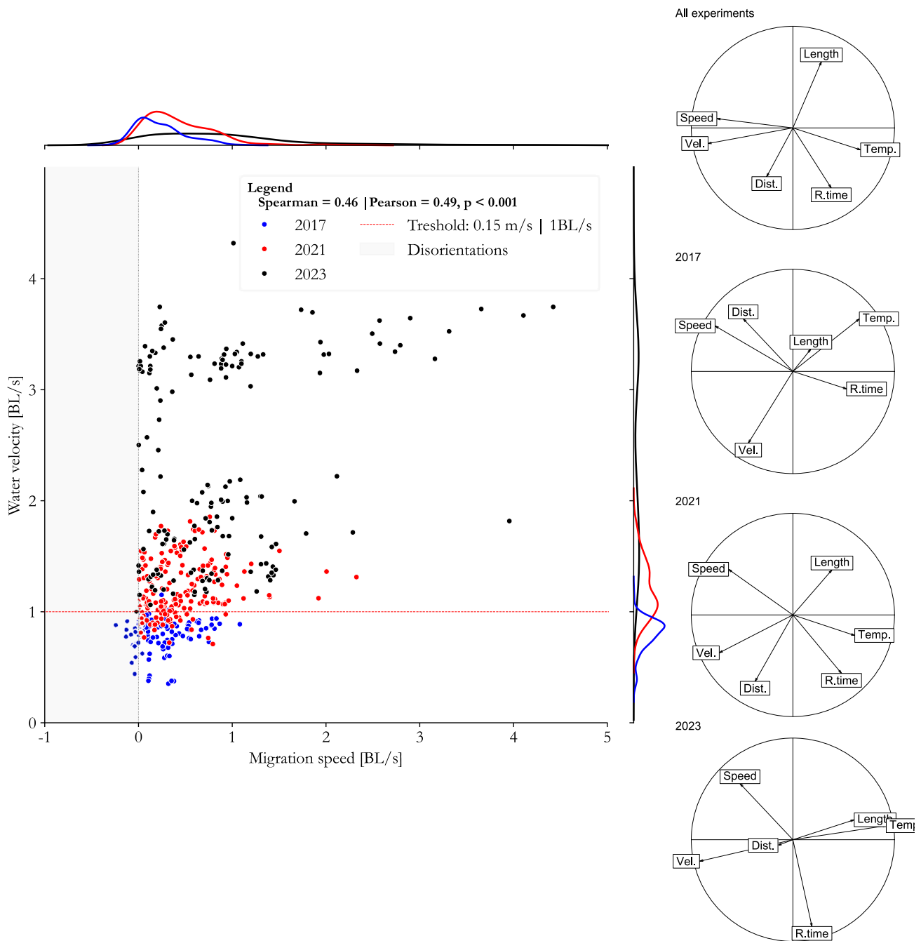
Fig. 8. Influence of water velocity on the migration speed of smolts. Correlation circle explain the relationships between variables with (R. speed: smolt relative speed, Vel.: average water velocity, Length: smolt length, Temp.: average water temperature, Dist.: distance already migrated by the smolt, R.time: average research time near obstacles).
