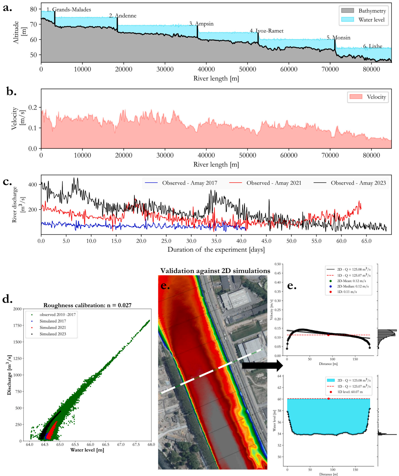
Fig. 3. The 1D model. With, a. Simulated water levels along the 82 km of the mid-lower Meuse River for a given time step, b. Simulated water velocities for the same time step, c. Observed hydrographs at Amay hydrometric station during the three experiments, d. Calibration of the friction coefficients used in the 1D model, e. Validation of the 1D simulated results against existing 2D simulations.
