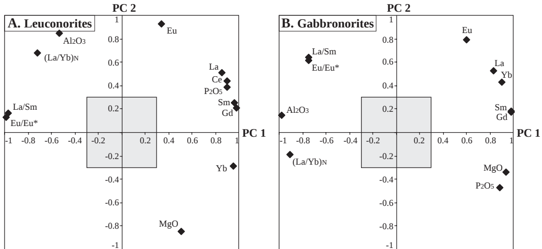
Fig. 5. Graphical representation of the factor loading in the plane of the principal components PC1 and PC2 for (A) leuconorites and (B) gabbronorites.
