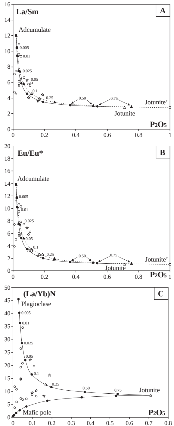
Fig. 9. (A) La/Sm vs. P 2 O 5 and (B) Eu/Eu* vs. P 2 O 5 for leuconorites and jotunite with mixing lines between bulk adcumulate and jotunite with the relative percentage of jotunite. Jotunite (△) is the proposed parental magma of BSKS (Duchesne and Hertogen, 1988) and Jotunite' (□) has the same REE content with 1% P 2 O 5 (see Table 6). (C) (La/Yb) N vs. P 2 O 5 for leuconorites with mixing lines plagioclase–jotunite and orthopyroxene–jotunite with the relative percentage of jotunite. Stars are samples from the north-eastern part (Teksevatnet area) and open circles (○) are from other localities.
