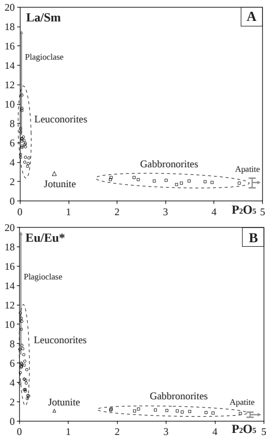
Fig. 8. (A) La/Sm vs. P 2 O 5 and (B) Eu/Eu* vs. P 2 O 5 for bulk cumulates (leuconorites—open circles (○) and gabbronorites—open squares (□) and jotunite—open triangle (△) with the range of composition for plagioclase and apatite indicated by the arrow.
