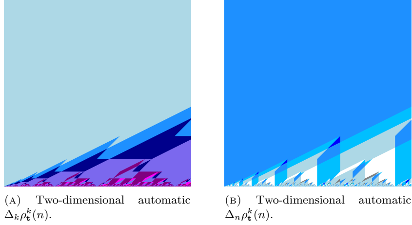
FIGURE 1. The Tribonacci sequence has bounded discrete derivatives (first 4096 values, n on the horizontal axis, k on the vertical axis, one color per value, a different palette for each picture).
