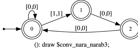
FIGURE 2. The converter between the Dumont–Thomas numeration systems associated with the Narayana substitution \tau and the substitution behind the length-3 sliding-block code of its fixed point (here it computes the identity).
