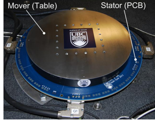
(b) Stage with infinite R_z rotation [42]
