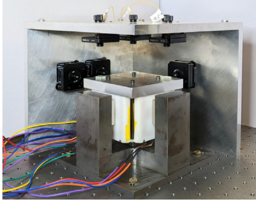
(a) LevCube with \approx 1 \text{ cm}^3 mobility [62]
