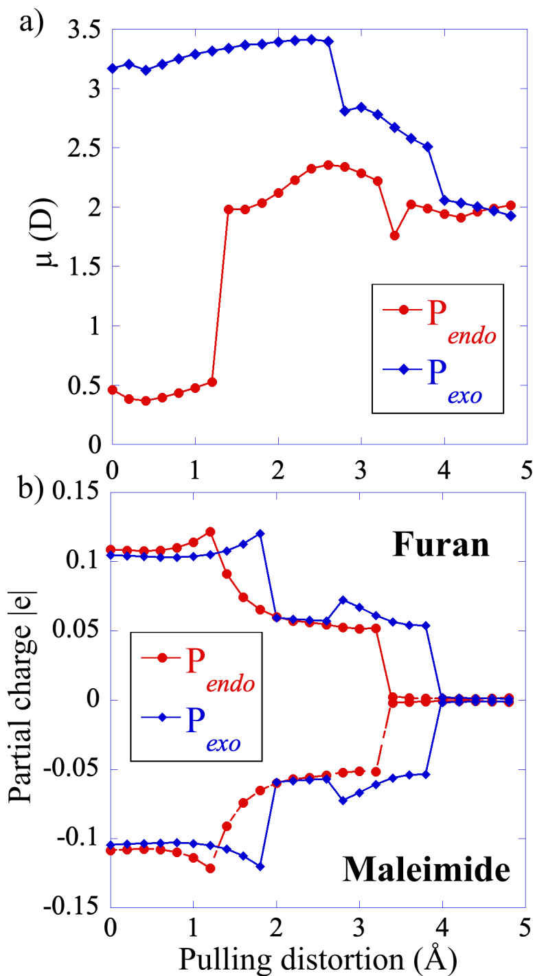
Figure 5. a) Permanent dipole of the two adducts along the CAS(4,4) CoGEF path for P_{endo} (red-filled circles) and P_{exo} (blue-diamonds). b) Computed partial charge on the furan and maleimide addends along the CAS CoGEF path.
