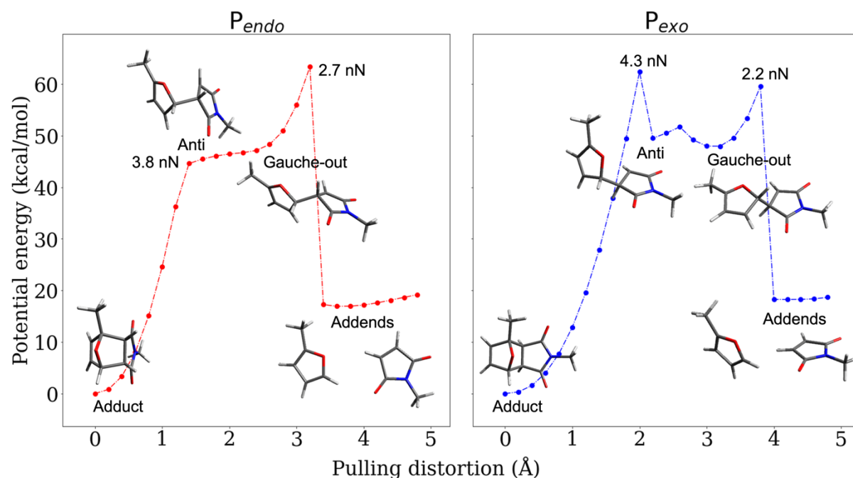
Figure 2. CoGEF UDFT wB97XD potential energy profiles for the P_{\text{endo}} (a) and P_{\text{exo}} (b) adducts as a function of the pulling distortion ( R_{\text{pulling}} - R_{\text{pulling-0}} ) as well as relaxed geometries under force for maxima and minima. The CoGEF path computed at the CAS(4,4) level is given in Figure S1 and the one computed with the PBE0DH and BH&HLYP functionals in figure S2. The relaxed geometries along the CoGEF paths computed at the DFT wB97XD and CAS(4,4) levels are given in the ESI.
