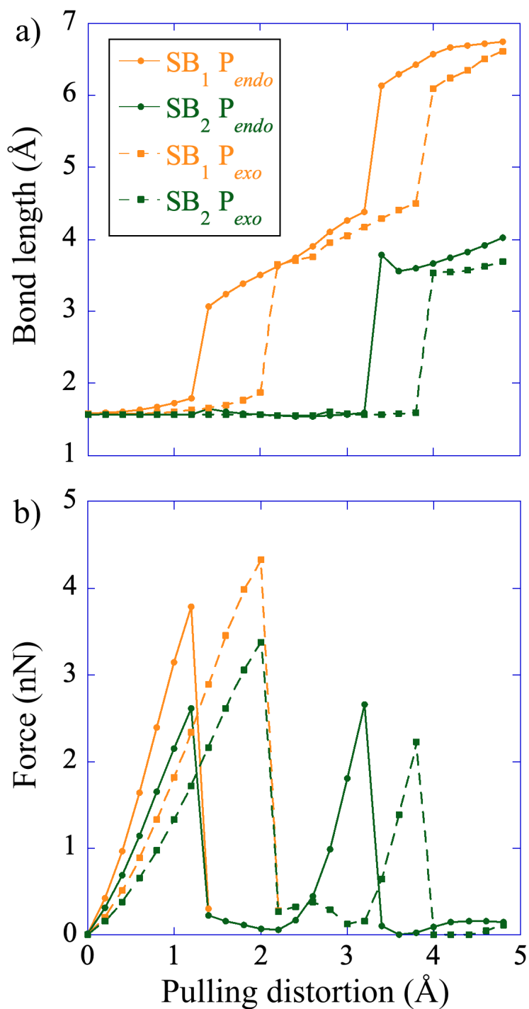
Figure 3. a) SB1 (orange) and SB2 (green) elongation plotted as a function of the pulling distortion for P_{endo} (full lines) and P_{exo} (dashes). b) Projection of the pulling force on SB1 and SB2 for the two adducts. The bond rupture and the maximum in the projection of the pulling force on the scissile bonds do not occur at the same value for P_{endo} and P_{exo} because of the difference in geometries of the two stereoisomers.
