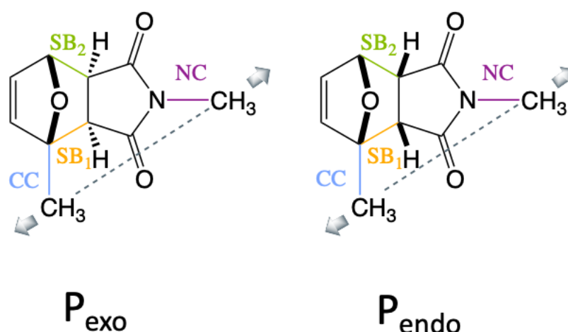
Figure 1. Stereochemistry of the P_{endo} and P_{exo} adducts, the labeling of the two scissile bonds, SB1 (orange) and SB2 (green) and of the two anchoring bonds, CC (blue) and NC (violet) and the direction of the stretching coordinate in dashes. The pulling coordinate has a larger projection on SB1 than on SB2.
