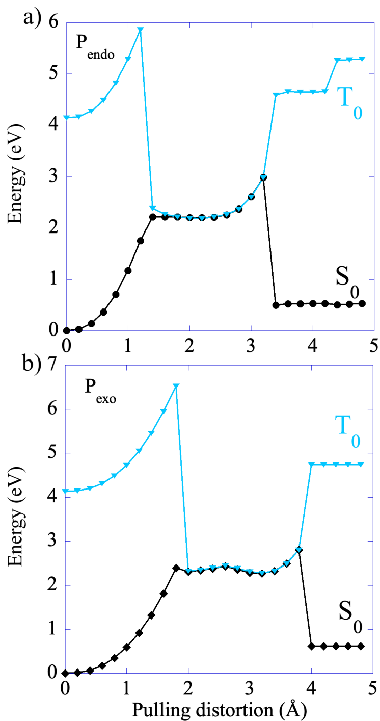
Figure 6. Energy profiles of the singlet S_0 and the lowest triplet T_0 along the CAS(4,4)-CoGEF path. The energy of the T_0 state is computed at the relaxed geometry of S_0 . The values of the spin-orbit coupling are reported in Table S1 of the ESI. The S_0/T_0 energy differences are plotted in Figure S6 and the minimum energy intersystem crossing (MEIC) geometries in Figure S7. Files of geometries of the S_0 state along the CoGEF path as well as at the MEIC are given in the ESI.
