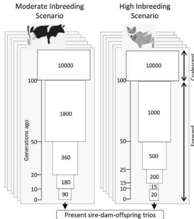
Figure 2. Simulated demographic scenarios. We simulated a moderately inbred population corresponding to a typical livestock population (e.g., dairy cattle), and a highly inbred population corresponding to an endangered wild population under conservation (similar to the Mexican Wolf). In both scenarios, we run a forward-in-time simulation with an initial population of N_e = 10,000 and equal sex ratio. In the moderate and high inbreeding scenario, the proportion of males for the subsequent generations was set to 0.1 and 0.5, respectively. The figure represents the evolution of N_e across generations.
