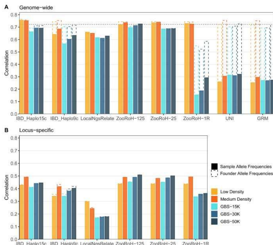
Figure 6. Impact of using founder versus sample allele frequencies on correlations between predicted and reference genome-wide (A) and locus-specific (B) HBD levels in the cattle data set, for the methods described in Table 1 that accept external allele frequencies as input. Reference inbreeding was estimated using the intermediate base population F mid. Correlations are shown for different marker panels including low-density, medium-density, and GBS panels with different
