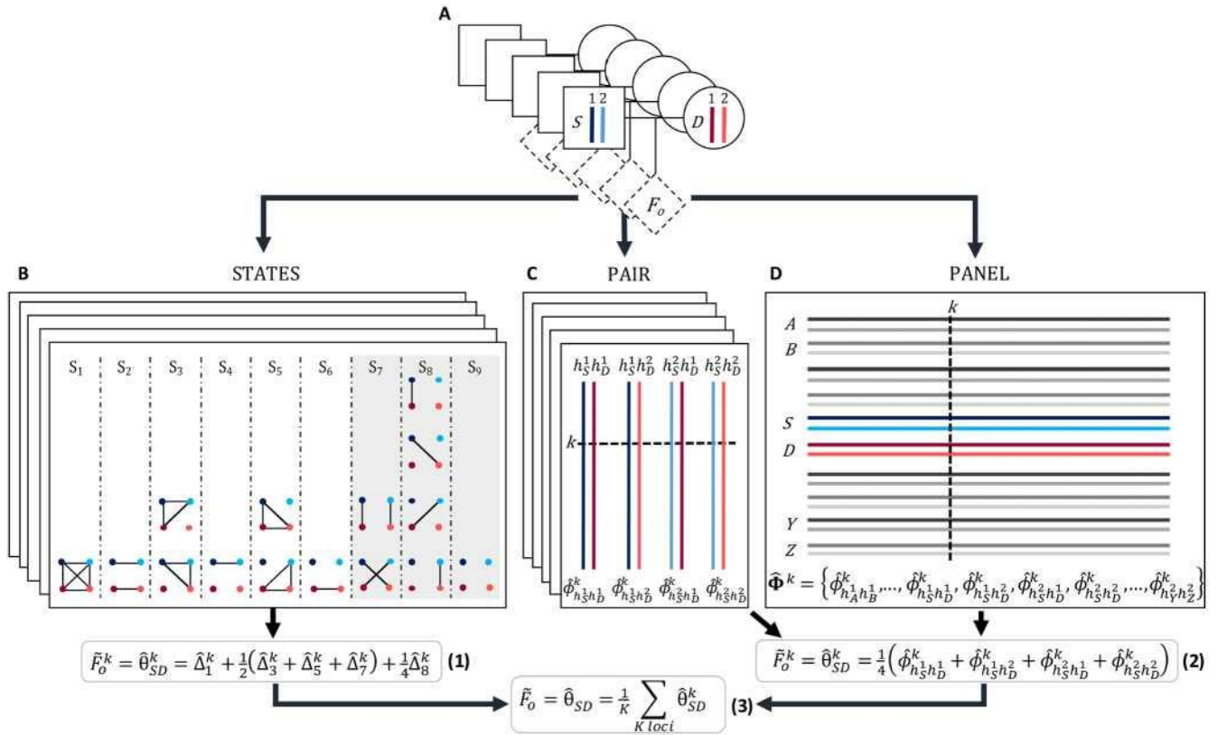
Figure 1. Approaches used to predict the homozygous-by-descent (HBD) level of an individual (FO) based on the genotypes of its parents. (A) Predictions were made in several trios, each including a sire (S) and a dam (D), having each a paternal and maternal haplotype (labelled 1 and 2, respectively), shown in blue for the sire and red for the dam, and the future offspring (dashed diamond). (B) STATES approach: For each pair of parents, the four parental haplotypes can take 15 possible identity-by-descent (IBD) configurations at a locus (Jacquard 1974). The four parental haplotypes are represented by dots using the same colours as in (A) while solid lines indicate IBD between linked haplotypes. Horizontal lines correspond to inbreeding within a parent, while vertical or diagonal lines indicate IBD between parents. The 15 IBD states can be grouped into 9 condensed IBD states \{S_1, S_2, \dots, S_9\} if the parental origins of the haplotypes within the two individuals are considered unknown. The number of states is reduced to three if the parents are assumed to be non-inbred (grey background). The STATES approaches model the observed genotypes or haplotypes conditional on these configurations. At locus k , the estimated probabilities of the 9 IBD modes \{\hat{\Delta}_1^k, \hat{\Delta}_2^k, \dots, \hat{\Delta}_9^k\} can be used to estimate the locus specific coancestry between the parents \hat{\theta}_{SD}^k (see also Lynch and Walsh 1998), which corresponds to the predicted locus-specific HBD level in the offspring \tilde{F}_O^k (Equation 1). (C) PAIR approach: IBD is modelled sequentially for each of the four possible combinations of parental haplotypes (h_S^1 h_D^1, h_S^1 h_D^2, h_S^2 h_D^1, h_S^2 h_D^2) , where h_I^1 and h_I^2 denote the paternal and maternal haplotypes of individual I , respectively. This analysis estimates the IBD probability \hat{\phi}_{h_S^i h_D^j}^k between two haplotypes h_S^i and h_D^j at locus k for the four possible pairs. (D) PANEL approach: A large panel of haplotypes from a large number of individuals are analysed jointly to detect IBD segments. At locus k , a vector \hat{\Phi}^k containing the IBD probabilities for each pair of haplotypes is estimated (note that with rule-based approaches, IBD probabilities are either 0 or 1). In the PAIR and PANEL approaches, the locus specific coancestry between the parents is obtained as the average over the four possible pairs of parental haplotypes (Equation 2). Finally, the genome-wide HBD levels \tilde{F}_O can then be predicted as the average locus-specific values at the K loci (Equation 3)
