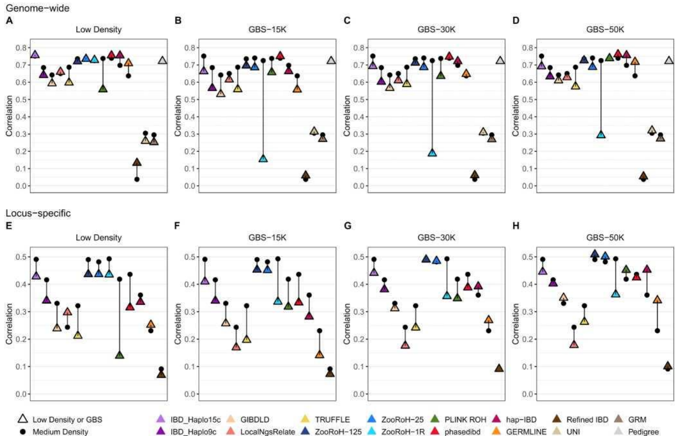
Figure 5. Correlations between predicted and reference genome-wide (A–D) or locus-specific (E–H) HBD levels for the 16 evaluated methods in the cattle data set using reduced genotyping arrays. Methods and their abbreviation are described in Table 1. Correlations obtained with low-density (A and E) or genotype-by-sequencing (GBS) (B–D and F–H) data were compared to those achieved with the medium-density array (triangles vs. dots). Reference inbreeding was estimated using the intermediate base population \hat{F}_{MID} .
