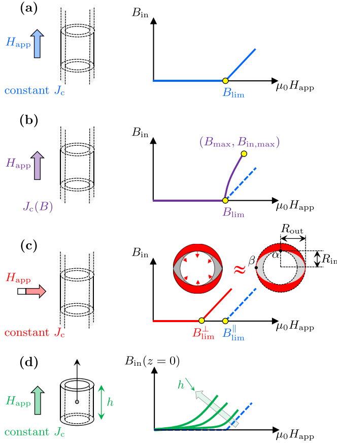
Figure 8. Schematic illustration of the internal magnetic flux density B_{in} as a function of the applied field \mu_0 H_{app} in different cases, along with a representation of the considered superconducting geometry. (a) infinite hollow cylinder with constant J_c subjected to an axial field, the curve serves as a reference and is shown as a dashed line for the three other panels, (b) infinite hollow cylinder with field-dependent J_c subjected to an axial field, (c) infinite hollow cylinder with constant J_c subjected to a transverse field, the cross-section of the cylinder schematically shows the nearly elliptical flux front reaching the inner wall of the cylinder, (d) finite hollow cylinder with constant J_c subjected to an axial field.
