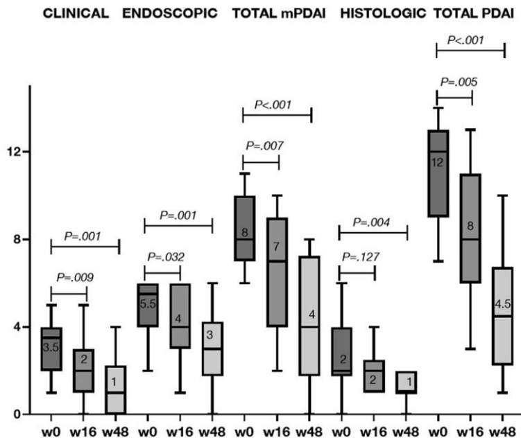
Figure 1. mPDAI and PDAI evolution. N at w0 = 22; n at w16 = 21; n at w48 = 14.
