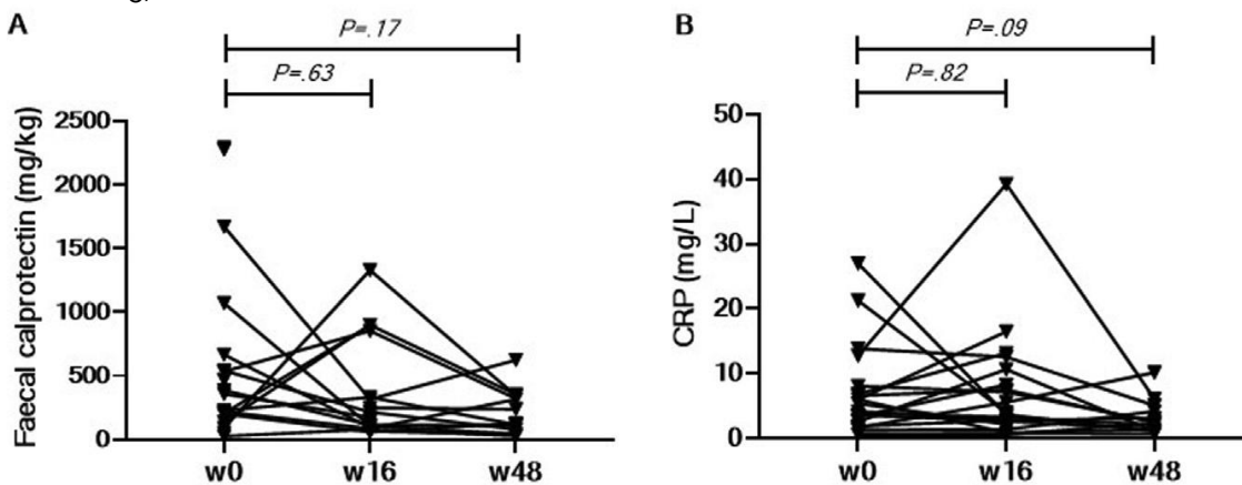
Figure 2. Fecal calprotectin (A) and CRP evolution (B). (A) n at w0 = 19; n at w16 = 17; n at w48 = 13. (B) n at w0 = 22; n at w16 = 21; n at w48 = 14. Normal reference values: \leq 250 mg/kg for fecal calprotectin and \leq 5 mg/L for CRP.
