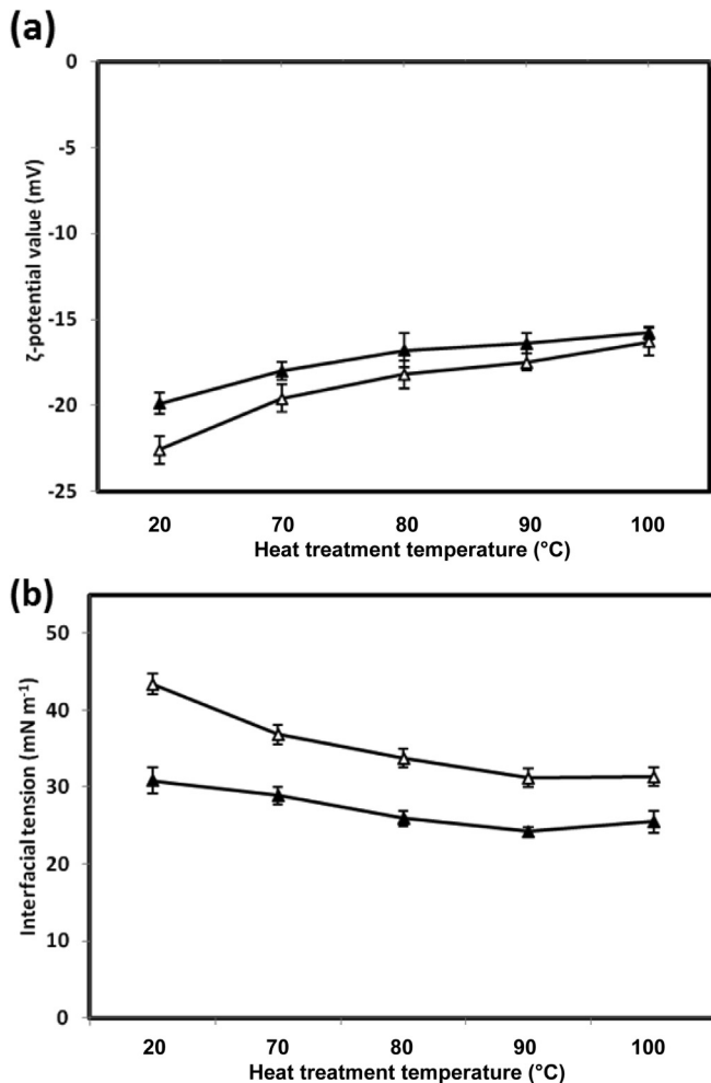
Fig. 7. \zeta -Potential (mV) (a) and the interfacial tension ( \text{mN m}^{-1} ) (b) of bovine and camel milk (at a protein concentration of 1 \text{ g L}^{-1} ) as a function of the heat treatment temperature; values are means \pm standard deviation ( n = 3 ).
