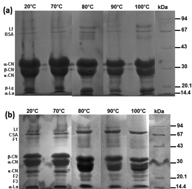
Fig. 6. SDS-PAGE electrophoresis patterns of bovine (a) and camel milk (b) proteins heated at 70 °C, 80 °C, 90 °C and 100 °C. Abbreviations are: CSA, camel serum albumin; BSA, bovine serum albumin; Lf, lactoferrin; \kappa -CN, \kappa -casein; \alpha -CN, \alpha -casein; \beta -CN, \beta -casein; F, fraction; \alpha -La, \alpha -lactalbumin; \beta -Lg, \beta -lactoglobulin.
