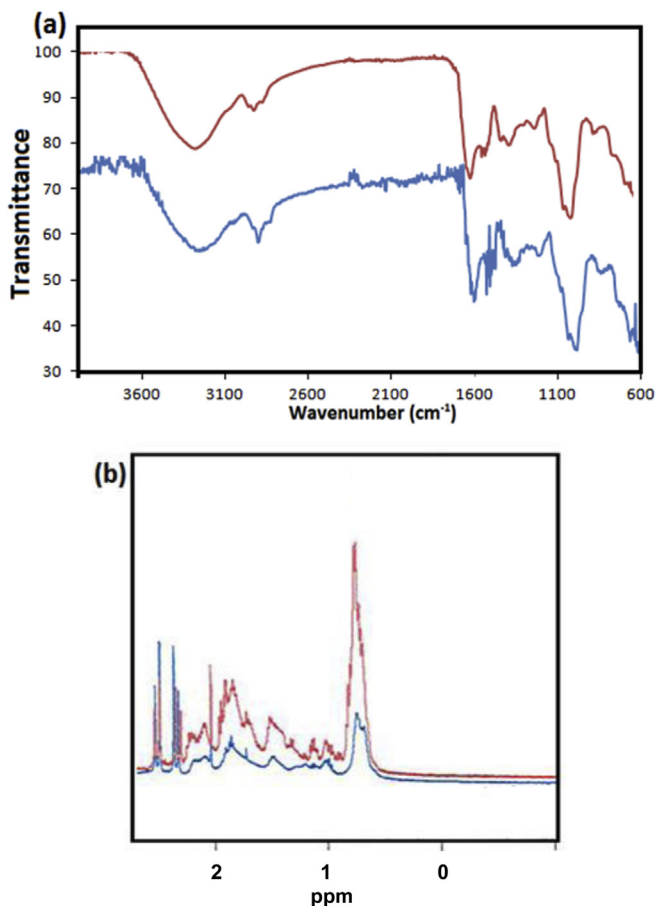
Fig. 3. FT-IR spectra (a) and ^1\text{H} NMR spectra (b) of purified camel \beta -casein (upper trace, red line) and bovine \beta -casein (lower trace, blue line) in their native state without any further modification. (For interpretation of the references to colour in this figure legend, the reader is referred to the Web version of this article.)
