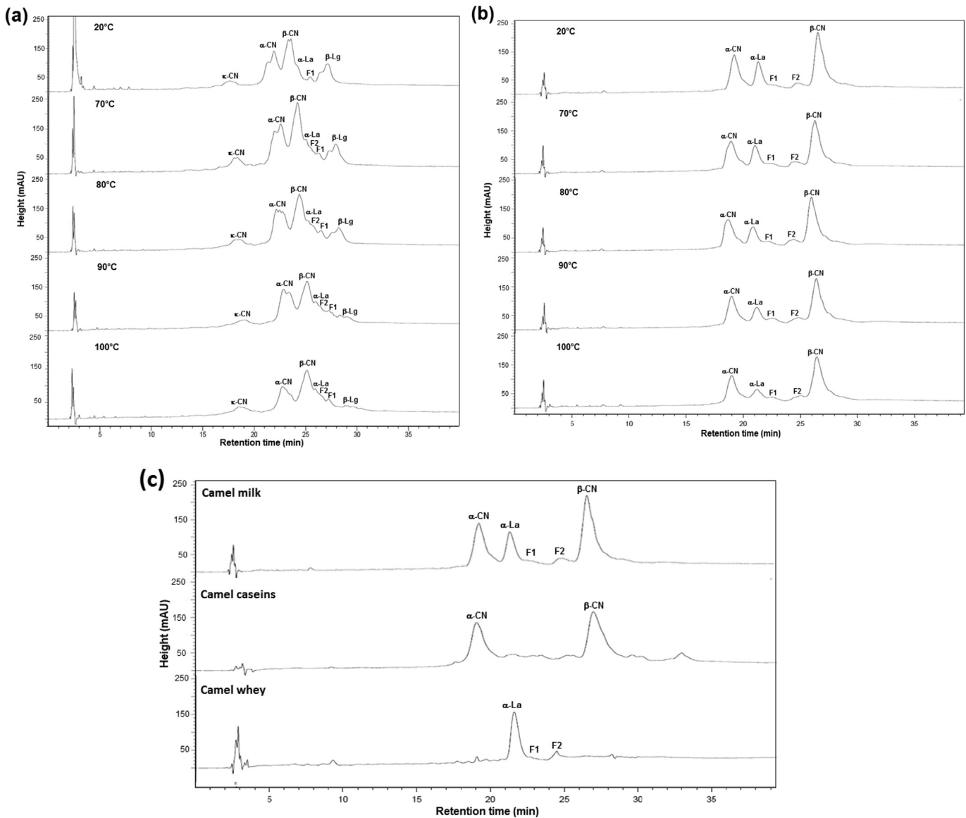
Fig. 5. HPLC chromatograms recorded at 220 nm for native (20 °C) and heated (70 °C, 80 °C, 90 °C and 100 °C) bovine milk and camel milk (panels a and b, respectively) and (panel c) camel milk, caseins, and whey chromatograms for camel milk protein identification. Abbreviations are: κ-CN, κ-casein; α-CN, α-casein; β-CN, β-casein; F, protein fraction; α-La, α-lactalbumin; β-Lg, β-lactoglobulin.
